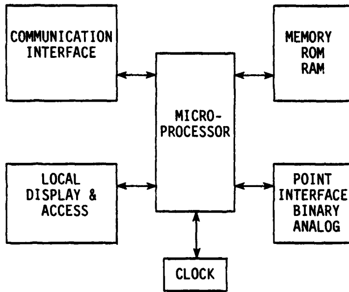
Figure 15. Digital controller hardware components.
