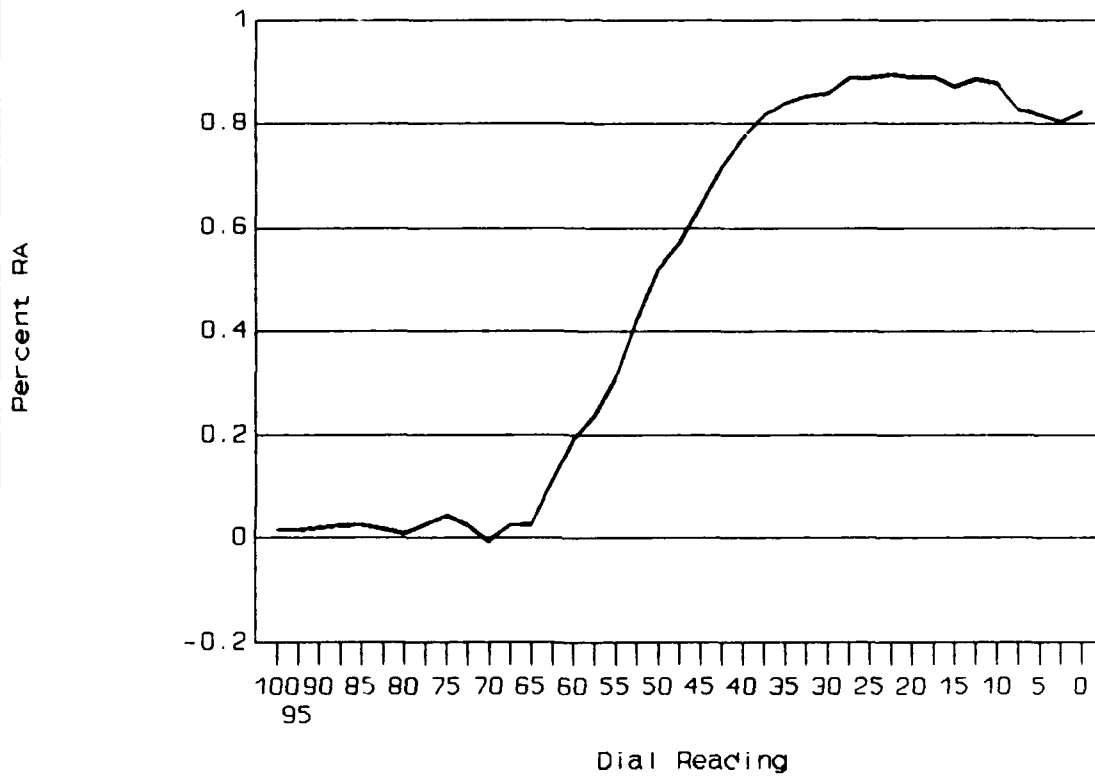
Figure 12. Percent Return Air (Decreasing Pressure)
