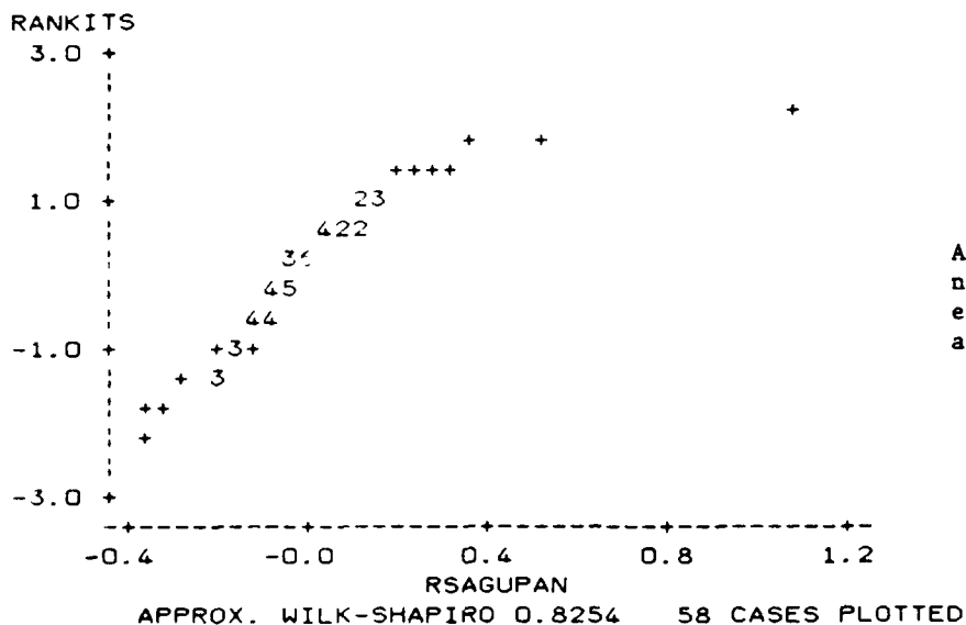
RANKITS VS RSAGUPAN
