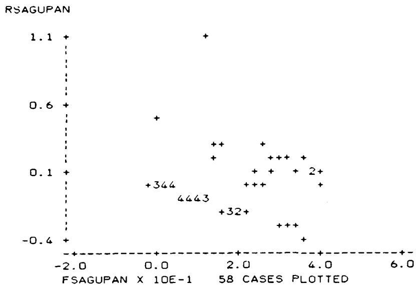
RSAGUPAN VS FSAGUPAN (STATISTIX)
