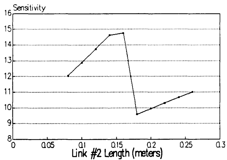
Figure 4-14 Sensitivity vs Link #2 Length
