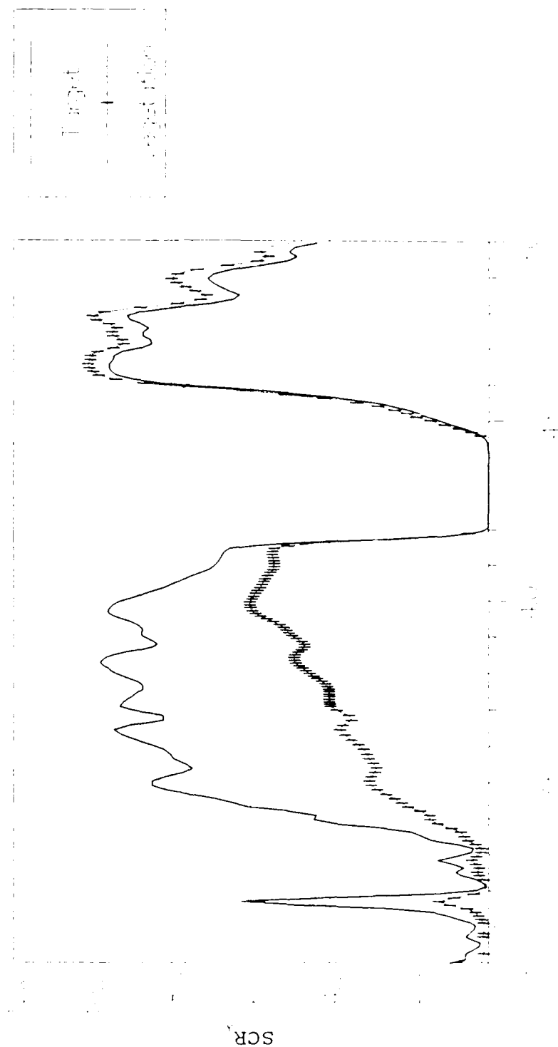
Figure 22. InSb Baseline Case, Vegetation, Day
