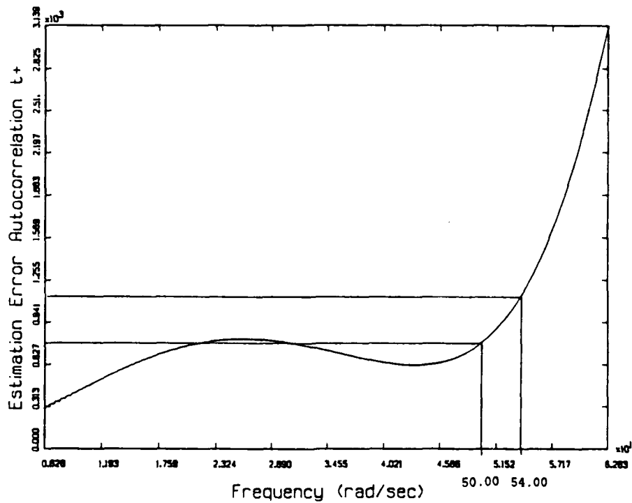
Figure 14. \hat{x}(t_i^+) Error Autocorrelation for Method 4, \omega_{nom} = 50.00
