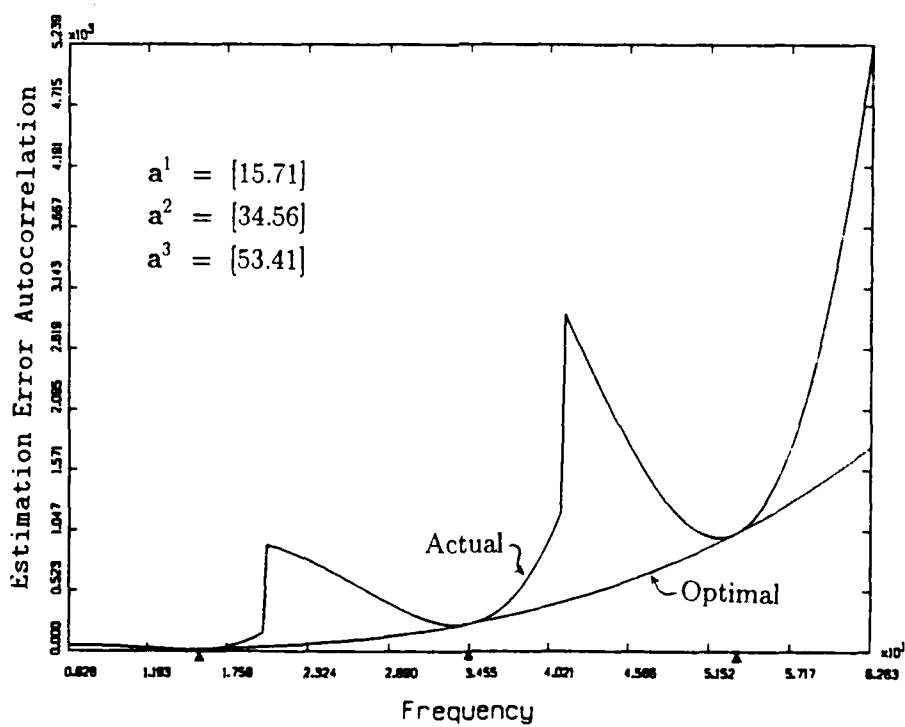
Figure 17. \tilde{x}(t_i^-) Autocorrelation Using Method 2
