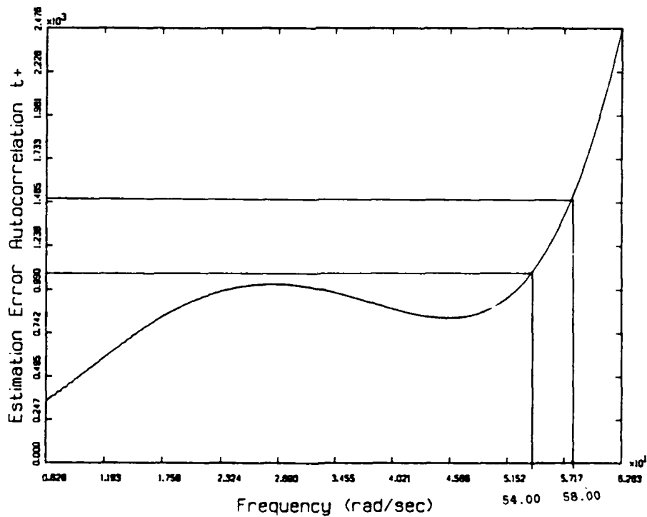
Figure 15. \hat{x}(t_i^+) Error Autocorrelation for Method 4, \omega_{nom} = 54.00
