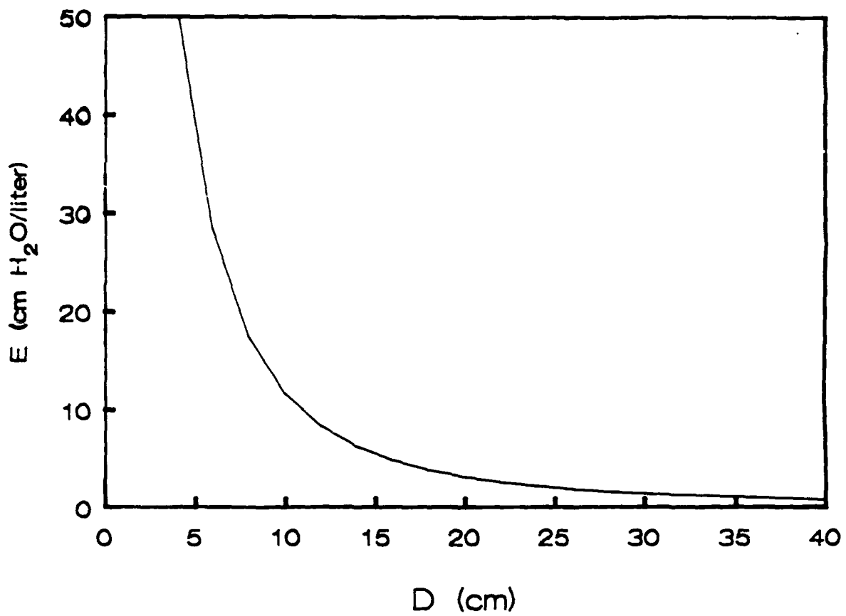
FIG. 13. VERTICAL CYLINDER MODEL PREDICTIONS: ELASTANCE vs. SIZE
