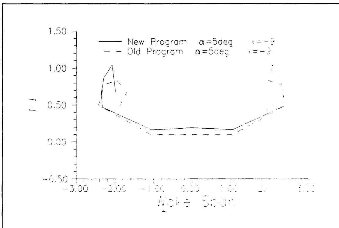
Figure 15d Wake Cross Sections (A.O.A. = 5 deg., x = -9 )
