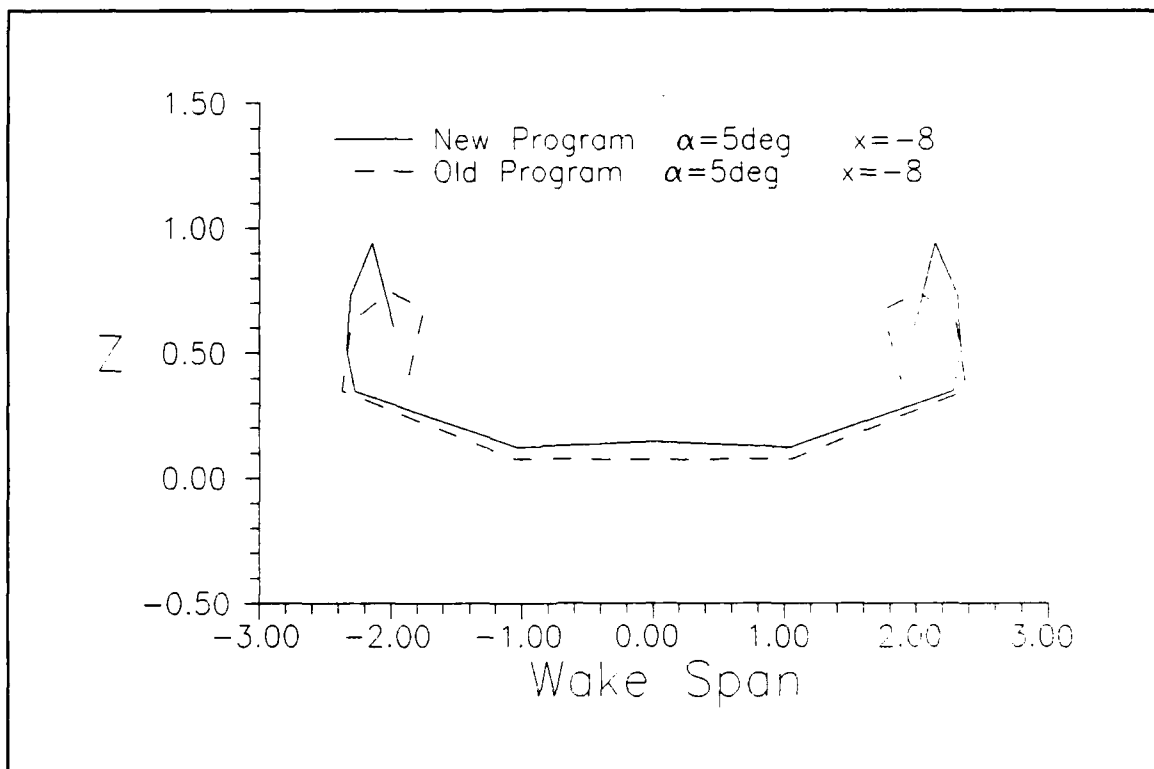
Figure 15c Wake Cross Sections (A.O.A. = 5 deg., x = -8 )
