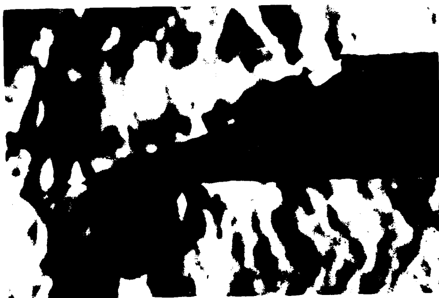
Figure 11a. Schlieren Photograph: Mach = 0.6, NPR = 2.0, BL Cowl
