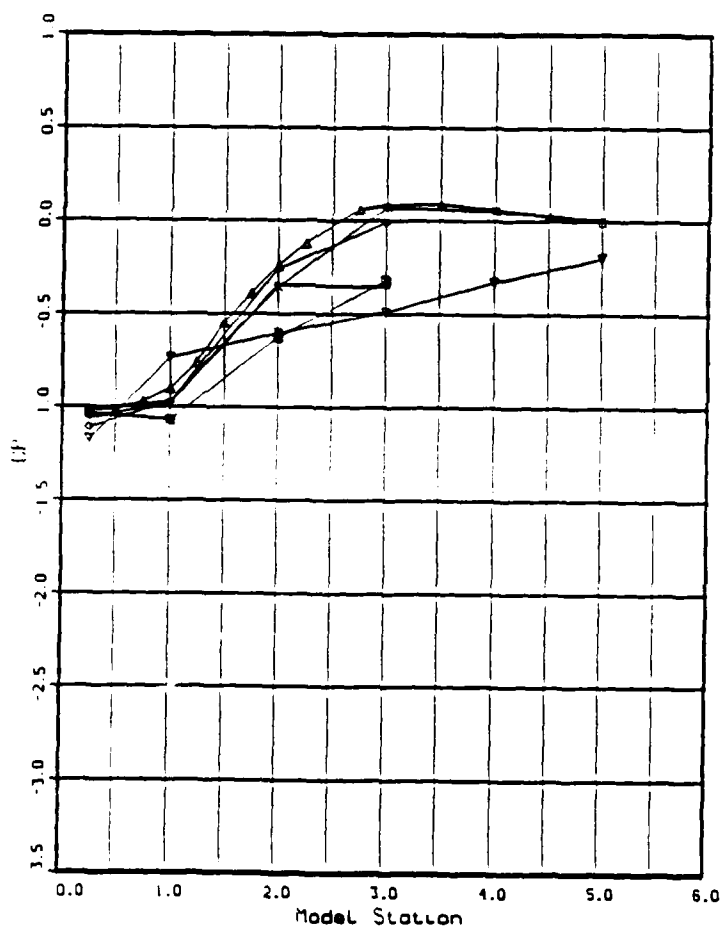
Figure B5. Surface Pressure Coefficients, C_p vs Model Station: Mach 0.8, NPR = 3.0, BL Cowl
