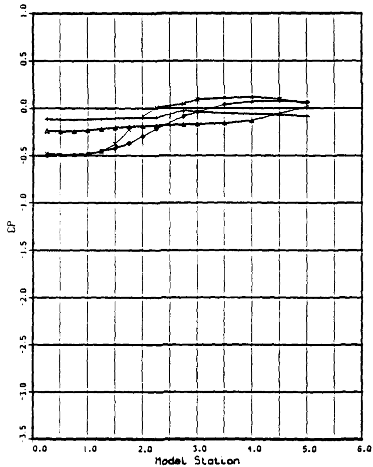
Figure 10a. Pressure Coefficient, C_p vs Model Station: Mach Number Effects, BL Cowl, NPR = 1.0
