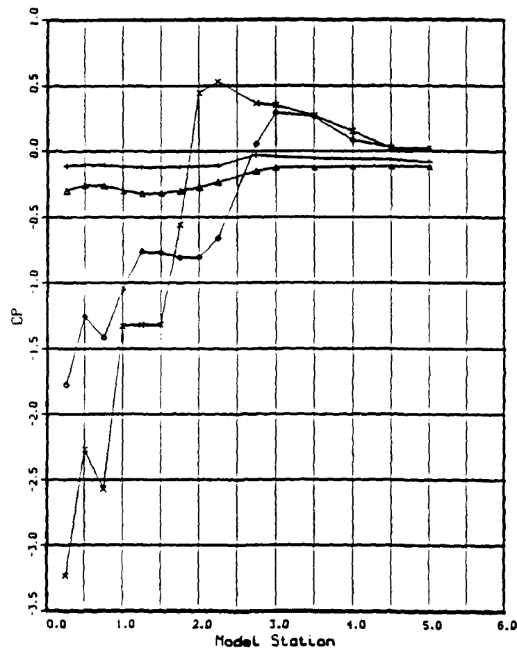
Figure 10c. Pressure Coefficient, C_p vs Model Station: Mach Number Effects, BL Cowl, NPR = 5.0
