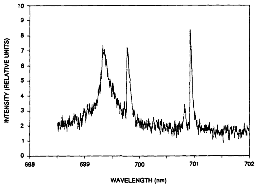
Figure 26. Optogalvanic spectrum of a nitrogen/argon DC discharge at 4.50 Torr.
