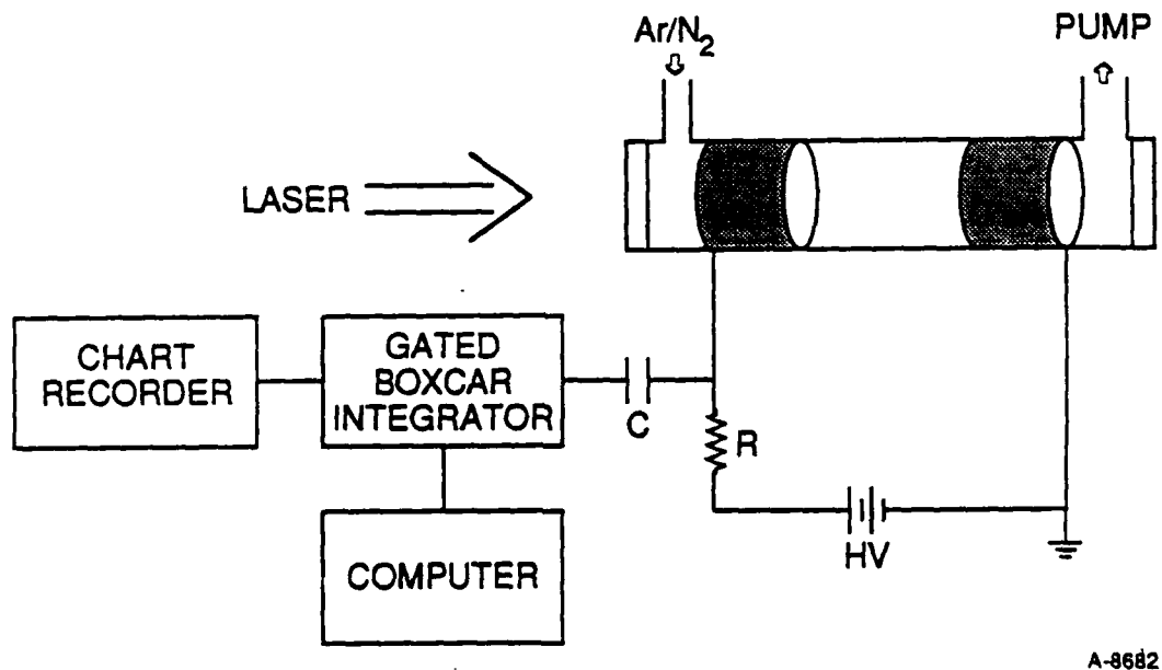
Figure 24. Experimental apparatus.
