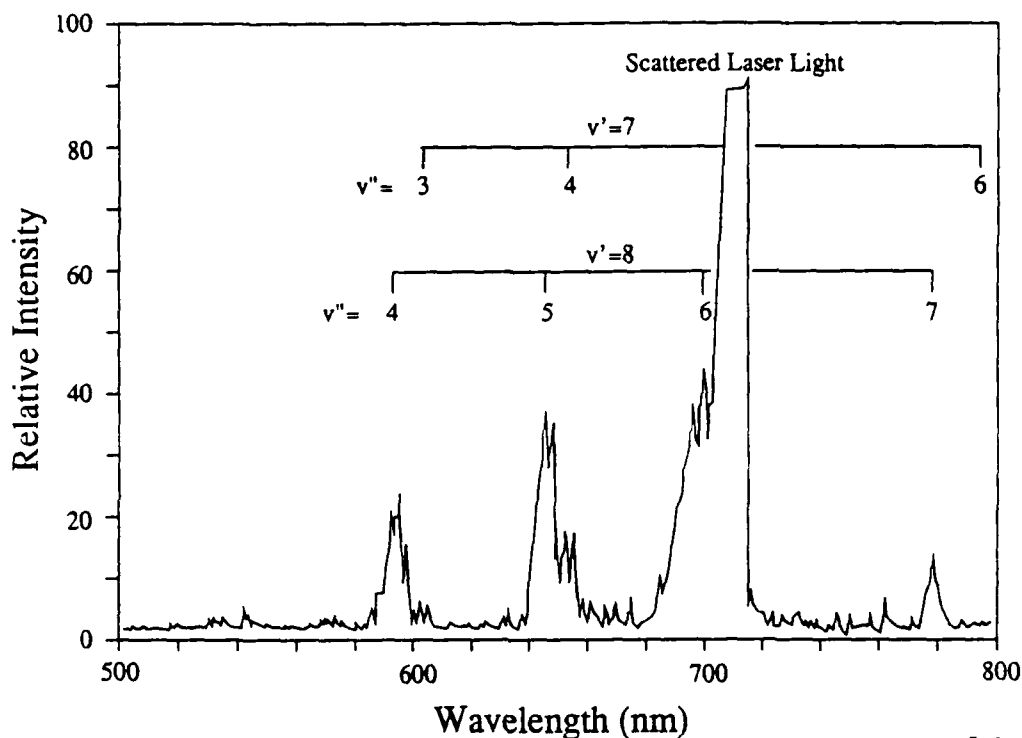
Figure 38. Resolved LIF spectrum for one of the absorption bands of Fig. 37. The features present can all be identified as originating from the B-A transition. Excitation of the 8,6 band is clearly indicated. Emission from B, v=7 is probably due to vibration relaxation of the B-state.
