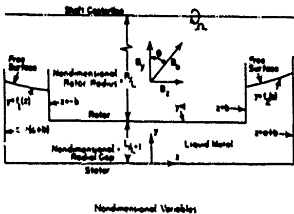
FIG. 1 Liquid-metal region between the stator and rotor. The coordinates and lengths are normalized by the radial gap length L .
