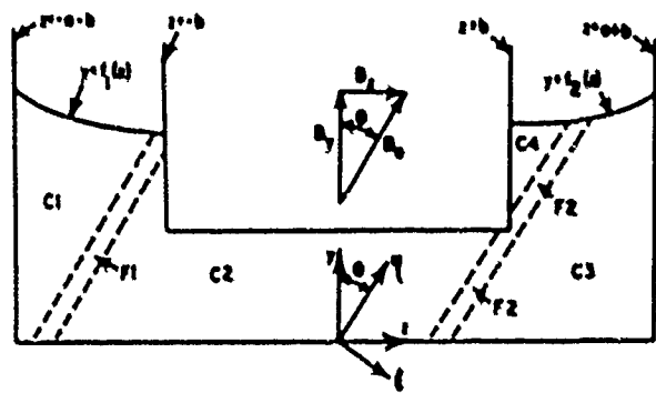
FIG. 5 Subregions of the liquid metal for M \gg 1 and general free-surface locations. The Hartmann layers and a weak free shear layer at \xi = -\sin \theta - b \cos \theta are not shown.
