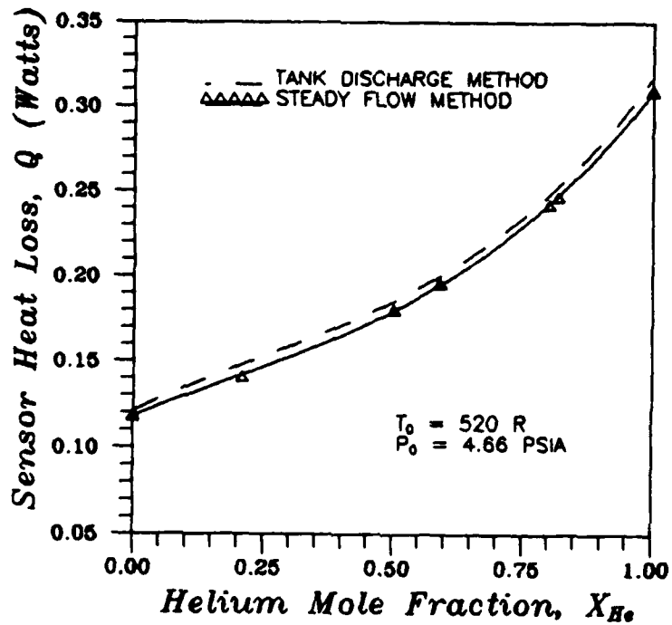
Figure 5.6. Calibration method comparison: steady flow vs. tank discharge
