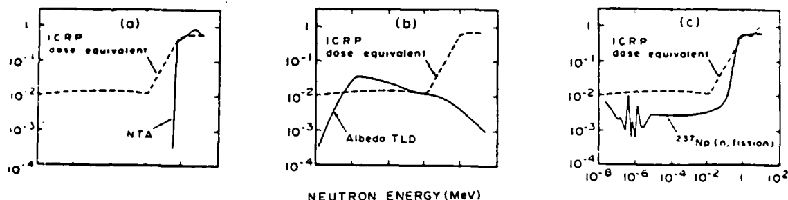
Figure 1.3 - Response of (a) NTA; (b) TLD; and (c) \text{Np}^{237}
