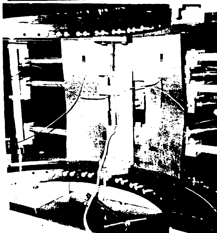
Fig 5.60 Pictures of 12" Unsupported Panel with 4" Cutout After to Collapse
