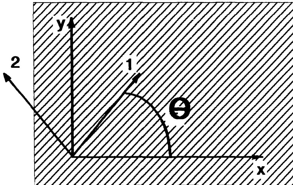
Fig E.2 Arbitrary Lamina Coordinates
