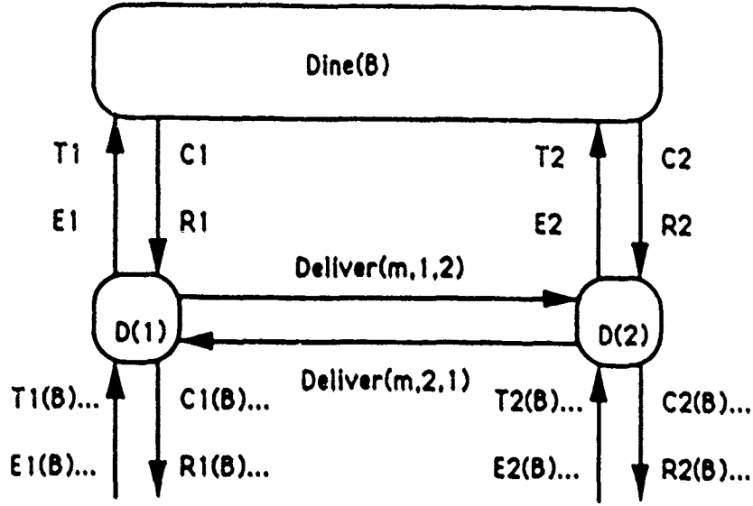
Figure 1: Drink(B) , a system of two drinking philosophers.
