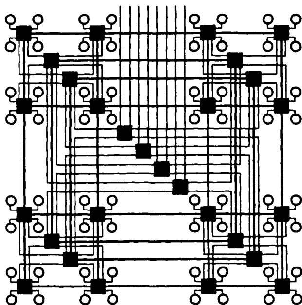
Figure 4-1: A fat-pyramid. This network is obtained by superposing hierarchical mesh connections on a butterfly fat-tree. The original fat-tree connections are represented by thin lines and the mesh connections by thick lines.
