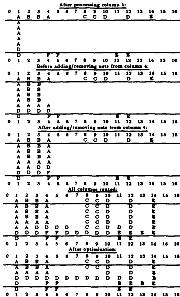
Figure 6-3: Shown is a plane as it appears at various points during the routing of the indicated channel. The routing of column 4 is shown both before and after the nets for terminals at the column are added or removed. Note the displacement of nets D, A and B that is caused by the entrance of net F. In addition, note how the exit of net F in column 5 allows net D to "drop" into the bottom row of the plane. The final optimization removes redundant rows, unnecessary doglegs (nets A and D) and excess wire runs (net C).
