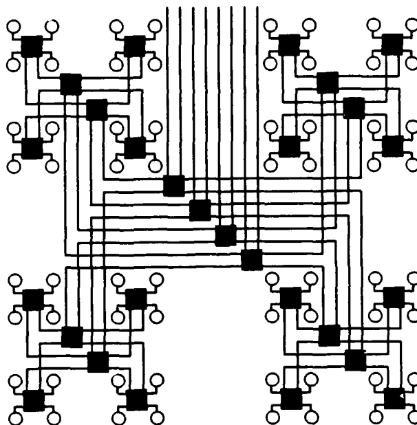
Figure 2-2: Another fat-tree design. The switches in this structure have constant size.
