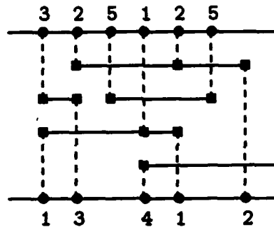
Figure 6-1: A representative channel routing problem in two layers. The horizontal wires (solid) are in one layer and the vertical (dashed) in the other layer. The vias are represented by squares and the terminals by circles.
