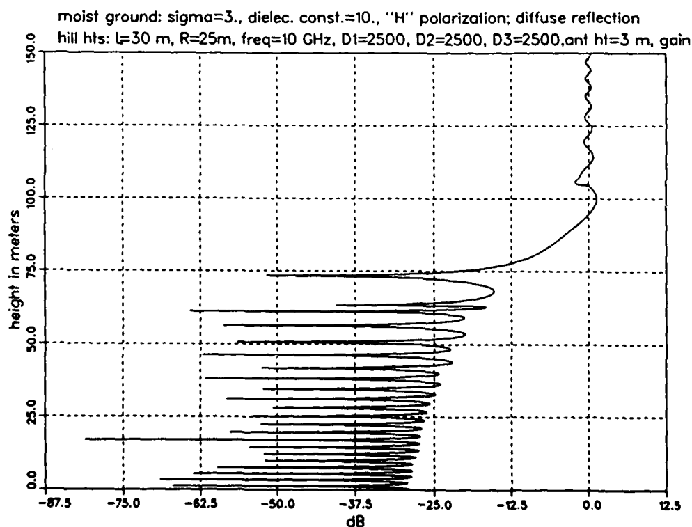
Figure D-14. Case of hill 30 m high near source and hill 25 m high near target, with horizontal polarization. Antenna height is 3 m.
