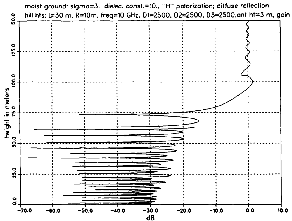
Figure D-11. Case of hill 30 m high near source and hill 10 m high near target, with horizontal polarization. Antenna height is 3 m.
