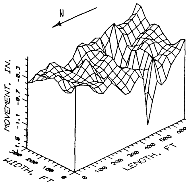
Figure 60. Three-dimensional view of mat movement
