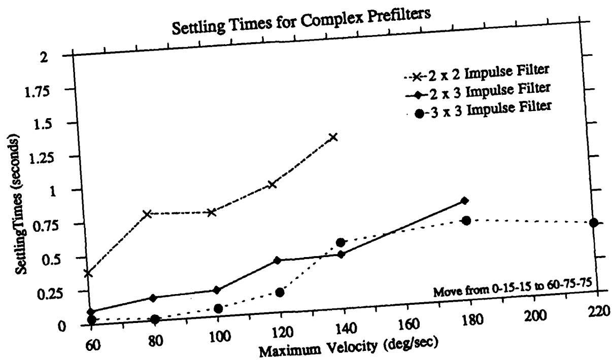
Figure 5.23: Complex filtering methods used on the complex move from 0-15-15 to 60-75-75.
