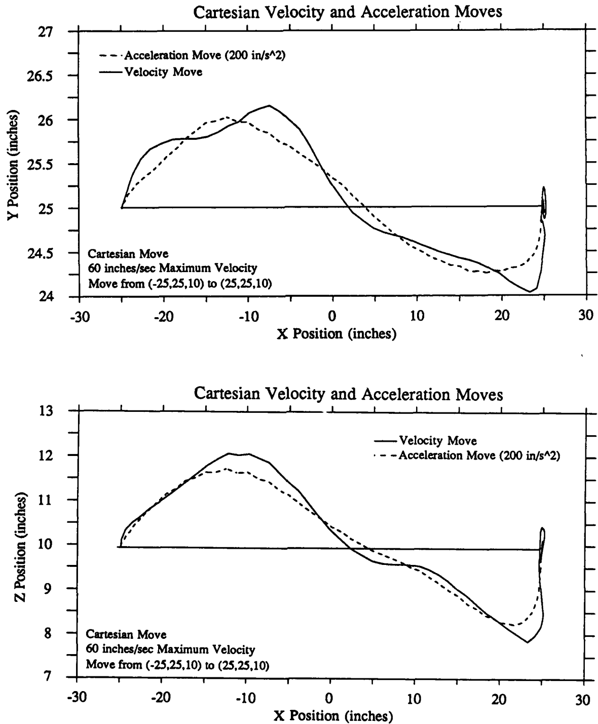
Figure 5.27: Trajectory followed by a velocity move and an acceleration move in cartesian space.
