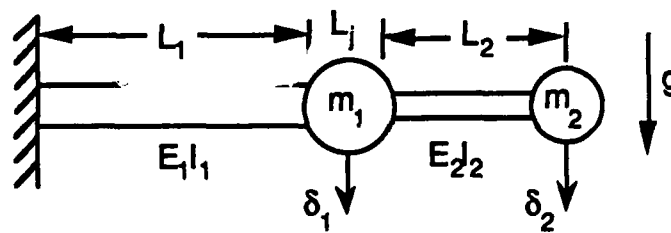
Figure 2.3: Two Cantilevered Beams with Masses
