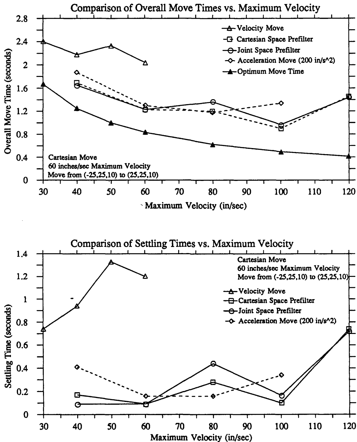
Figure 5.29: Comparison of different cartesian motion techniques.
