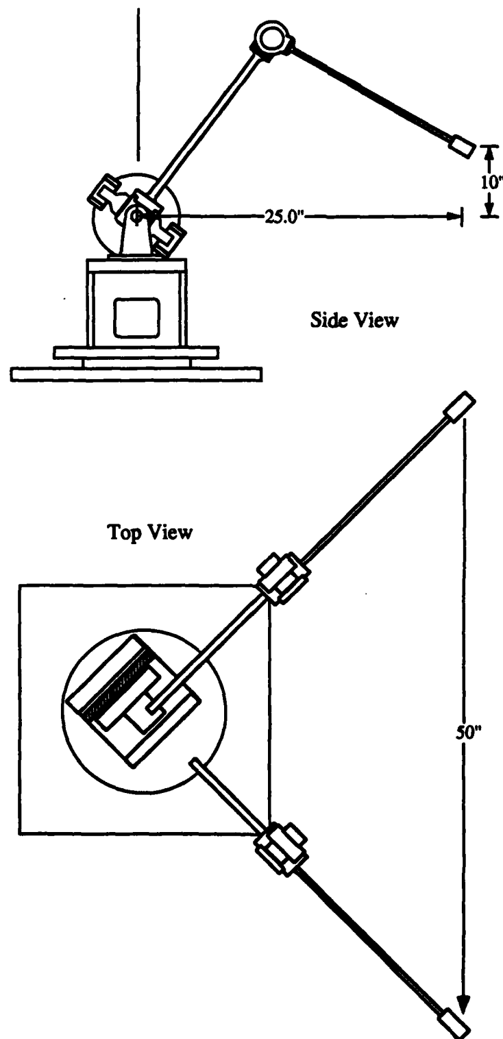
Figure 5.26: Configuration of the Flexbot for the cartesian motion. The payload of the robot moves in along the straight line between the start and stop positions.
