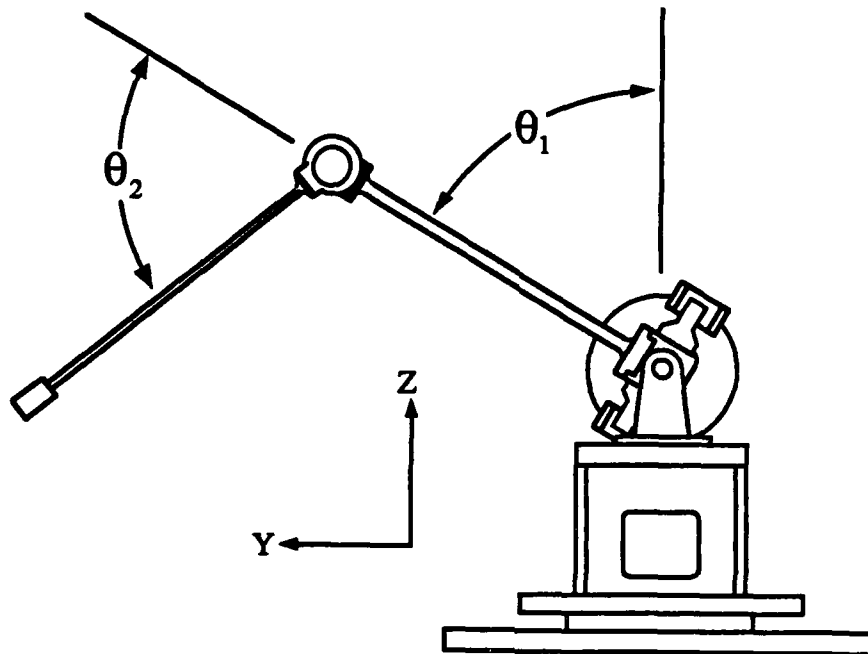
Figure 4.7: Joint positions for the Flexbot
