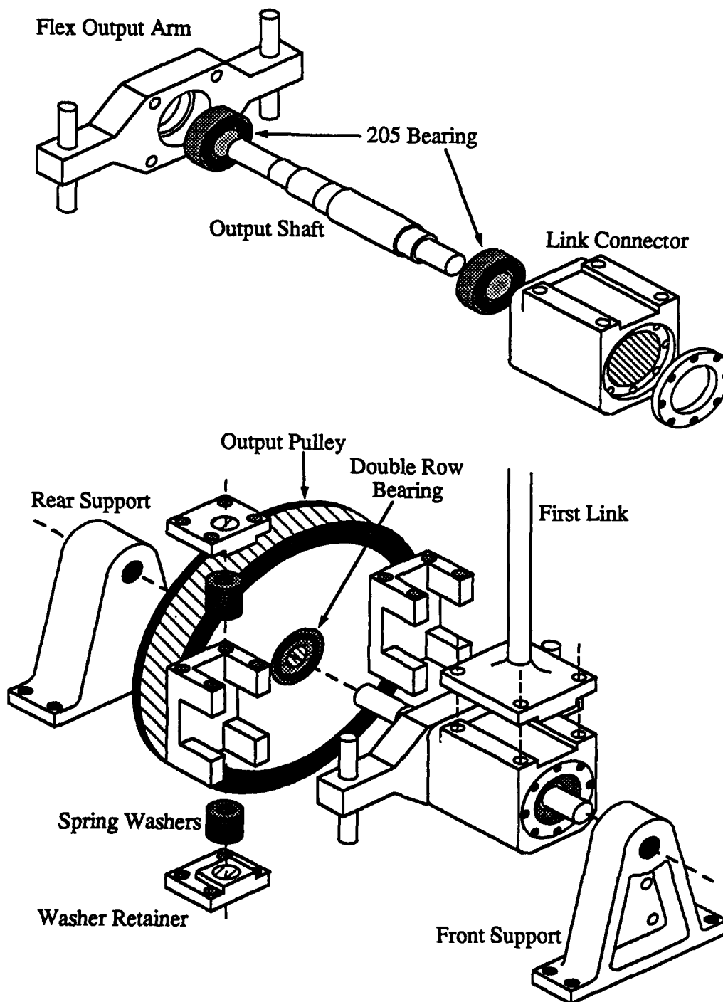
Figure 3.7: Exploded view of the output shaft of the first axis.
