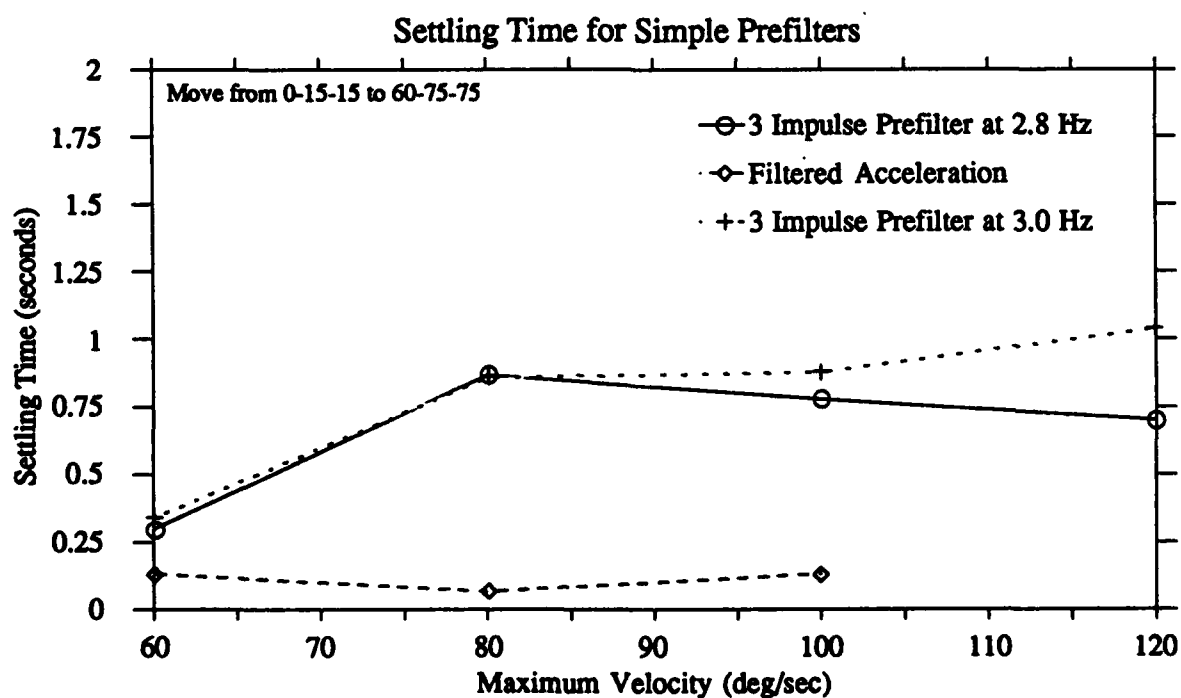
Figure 5.22: Simple filtering methods used on the complex move from 0-15-15 to 60-75-75. The filtered acceleration move is a combination of a three impulse prefilter at 2.8 hertz and an acceleration of 240 \text{ deg/sec}^2 .
