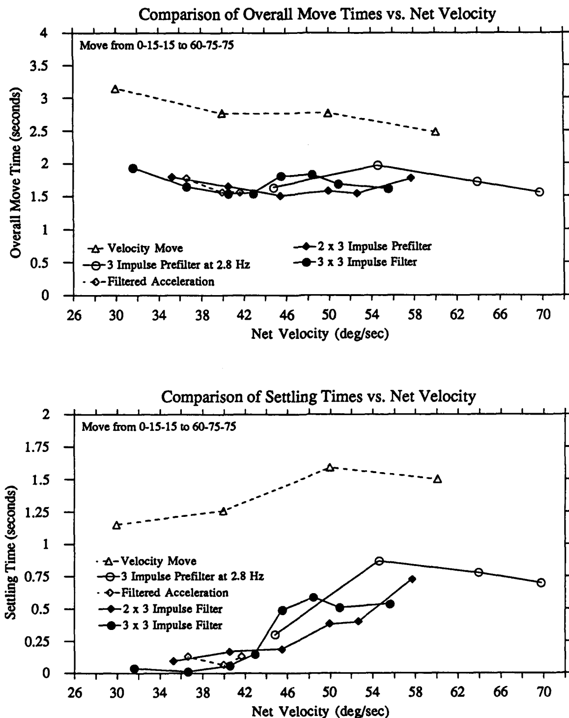
Figure 5.25: Comparison of the best methods for the complex motion from 0-15-15 to 60-75-75 against net velocity of the move.
