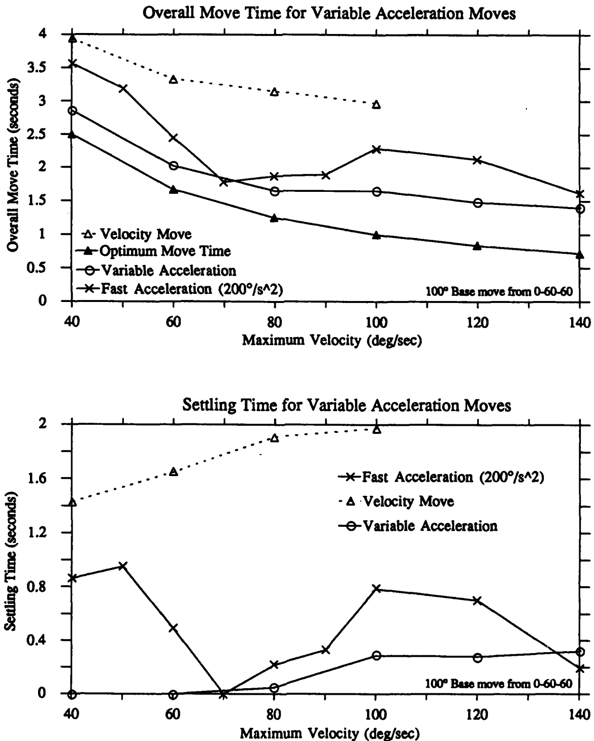
Figure 5.13: Variable acceleration move for a 100 degree move of the base joint with the first and elbow axes at 60 degrees apiece. The variable acceleration is compared against the constant 200 \text{ deg/sec}^2 acceleration move.
