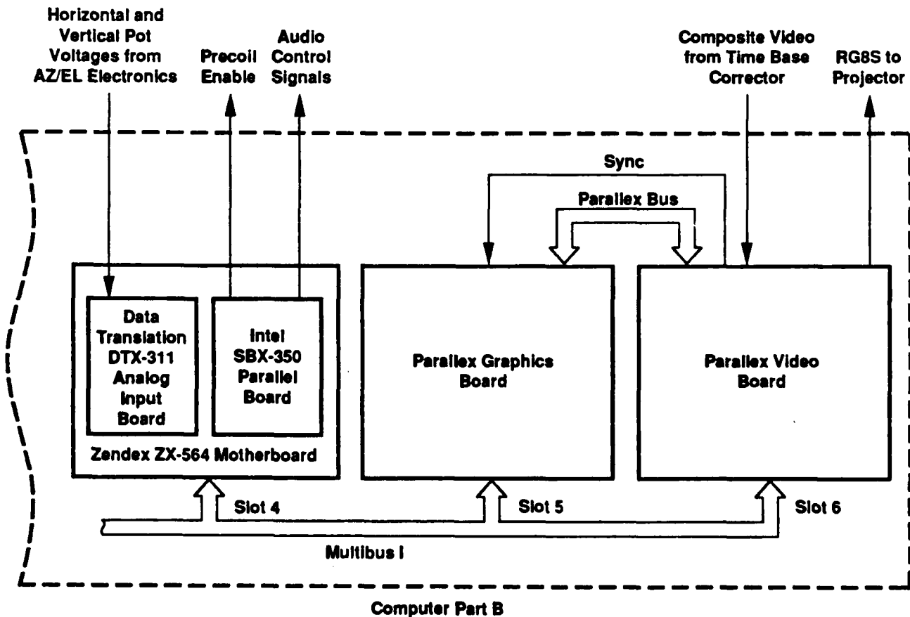
Figure 8. Computer sub-assemblies - 2.
