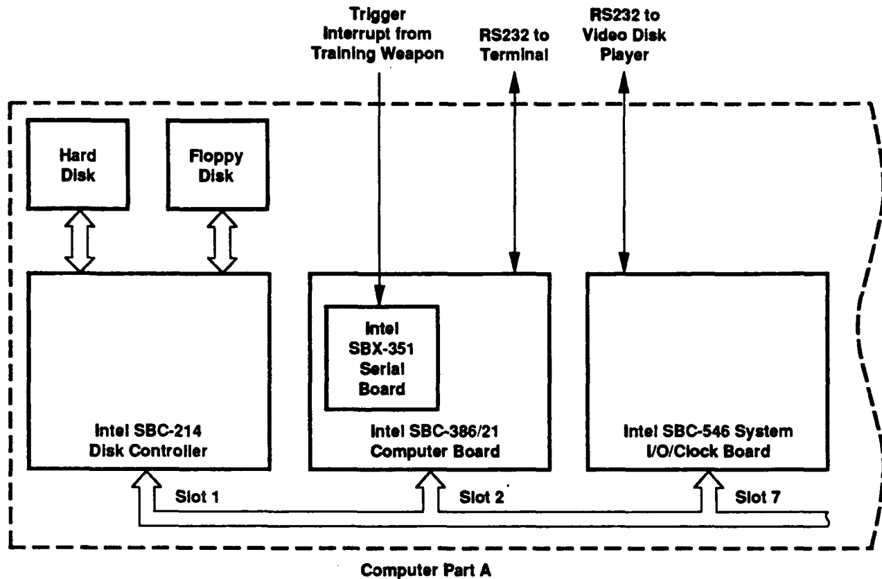
Figure 7. Computer sub-assemblies - 1.
