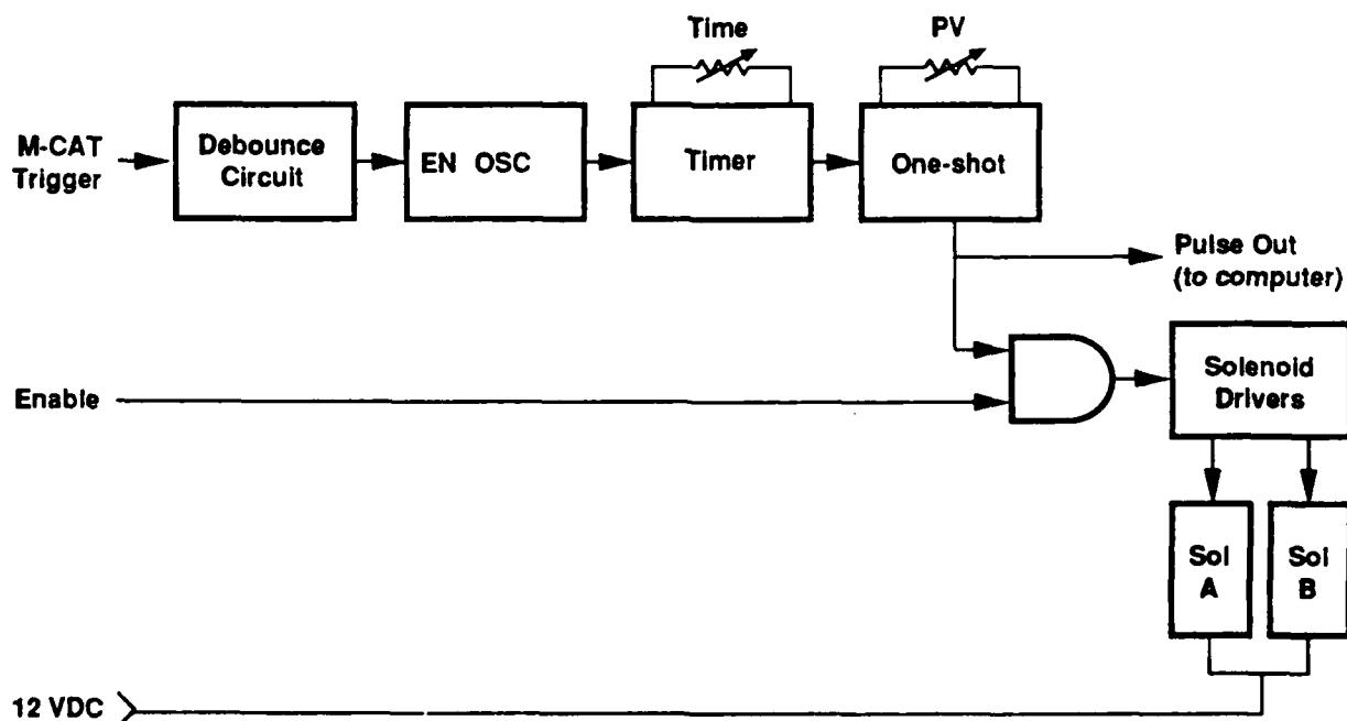
Figure 12. Recoil circuit.
