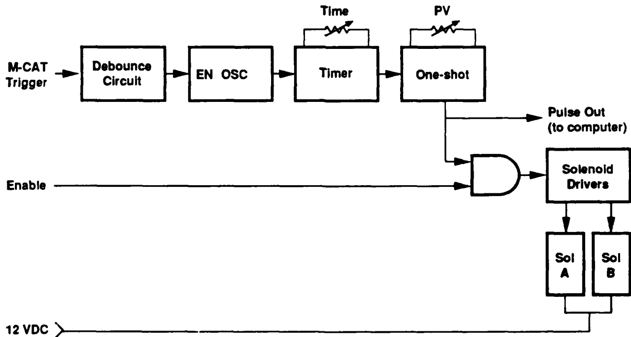
Figure 12. Recoil circuit.
