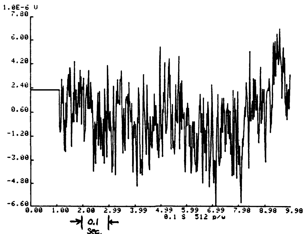
FIGURE 49. SYSTEM NOISE
