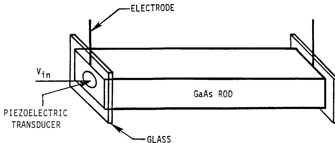
FIGURE 35. SEMI-CONDUCTOR GRATING
