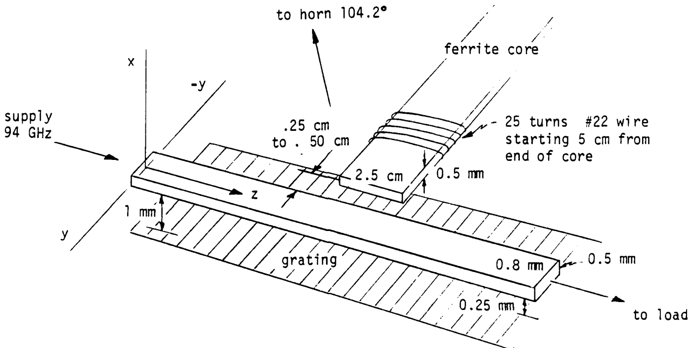
FIGURE 39. FERRITE WAVEGUIDE CONFIGURATION
