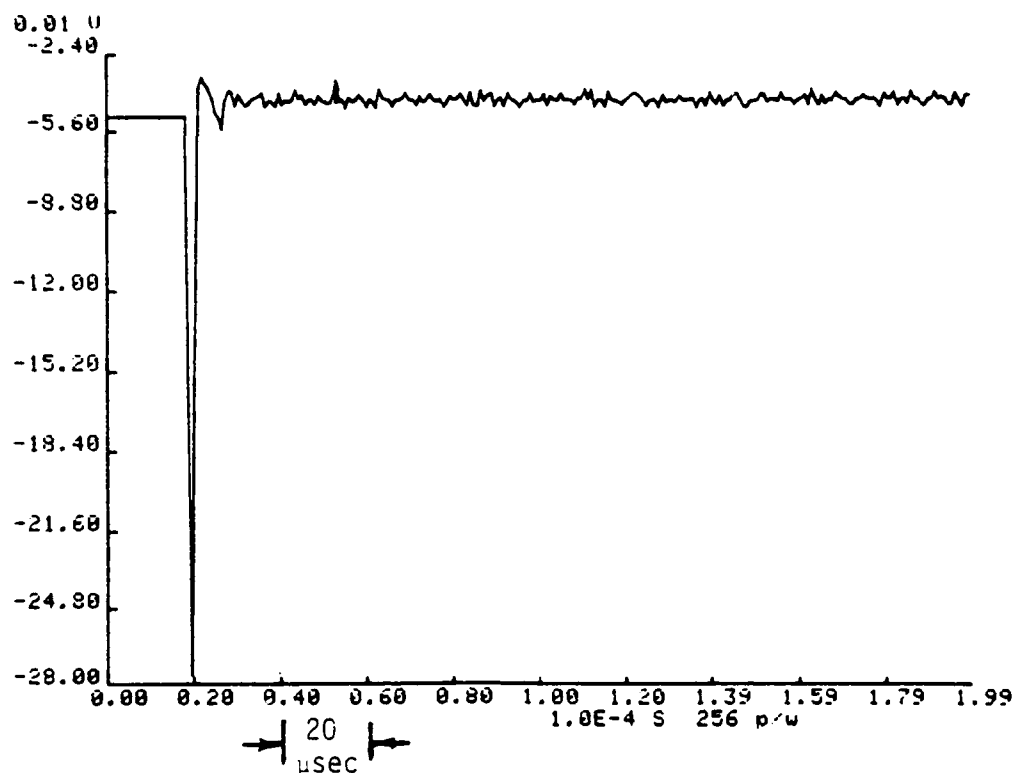
FIGURE 50. PHOTOCONDUCTIVE RESPONSE OF SILICON
