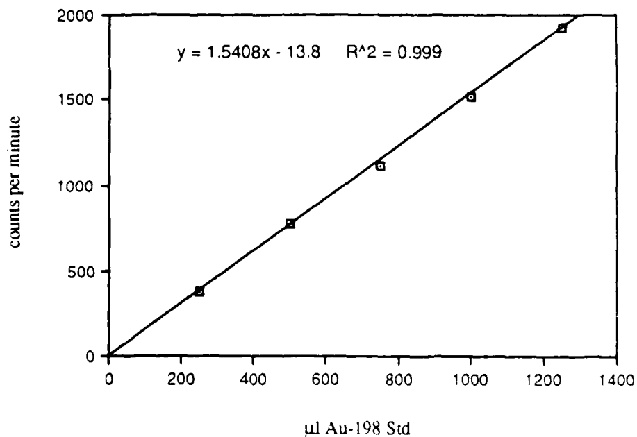
Figure 2.3: The plot is an example of testing whether count rate increased linearly with activity for a given geometry, solution volume and activity range. In this case, aliquots of ^{198}\text{Au} were diluted to 20 ml with 5% AR in 20 ml polyethylene vials and counted in the NaI(Tl) gamma counting system used for preliminary work. For the system description, see section 2.1.2.
