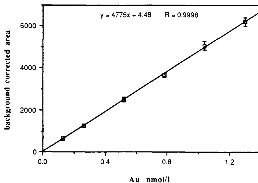
Figure 2.11: This is a plot of FI-ICPMS analysis (June 3, 1988) of Au standards in 5% AR. Each point represents the average of triplicate injections with 1\sigma errors. A 220 \mu l loop was used with instrumental parameters given in section 2.1.6.4 and Appendix C. Assuming 3\sigma of the background signal is 250 areal counts, an absolute detection limit of 10 fmol per injection is obtained.
