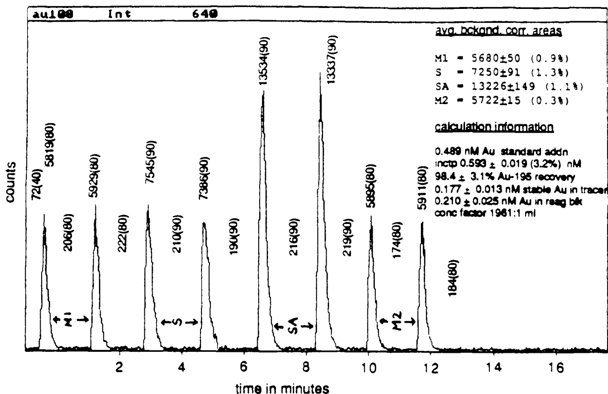
Figure 2.10: This is a plot of typical FI-ICPMS data output. The peaks represent transient signals for Au at mass 197 based on 120 \mu l injections. The standard was injected in duplicate before (M1) and after the sample (M2) and the sample was injected in duplicate (S) followed by a standard addition in duplicate (SA). Uncorrected areal counts for the number of channels in parentheses are given. The average of counts before and after a peak was used for background correction. Duplicates were then averaged and assigned a 1 \sigma error. The standard was checked for signs of instrumental drift and the data processed as described in Section 2.1.6.4. This particular sample was from the Black Sea and contained 110 \pm 20 fmol/l. See section 2.1.6 and Appendix C for instrumental operating conditions and section 2.2 for the preconcentration procedure.
