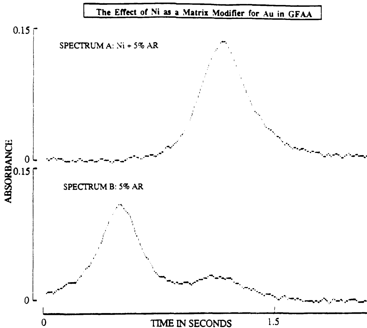
Figure 2.8: The spectra are graphite furnace atomic absorption peaks for Au (20 \mu l of 50 nmol/l Au in 5% AR) with and without Ni (0.52 \mu mol/ml sample) as a matrix modifier. The samples were atomized from a L'vov platform in a pyrolytically coated graphite tube under the conditions outlined in Appendix B for the ZGFAA system. It can be seen that, in the presence of Ni, the peak shape is nearly Gaussian whereas it is quite irregular for the AR only matrix. Refer to Section 2.1.5. for further discussion.
