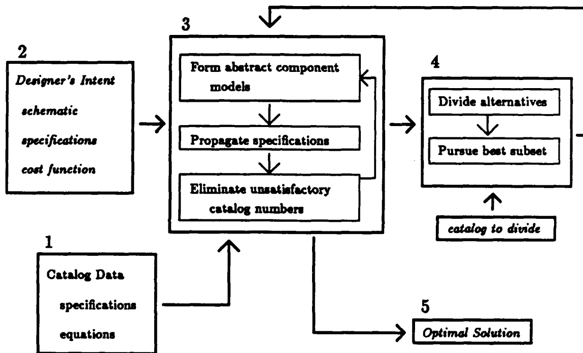
Figure 2.1: The Compiler Block Diagram
