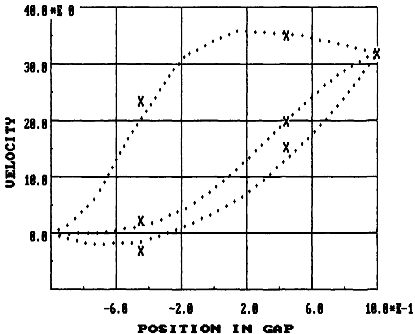
Figure 8. Velocity Profiles at Exit, Halfway & Entrance for Infinite-Width Slider, h_1/h_2 = 4 N=8 (...); N=2 (X)
