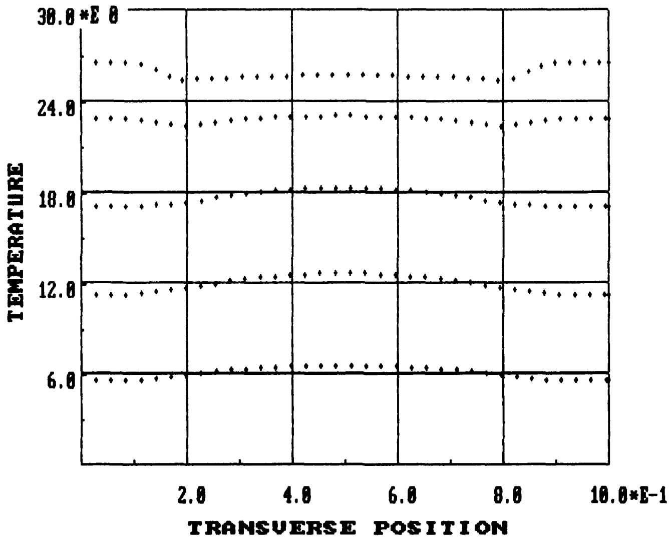
Figure 11. Center Temperature Profiles for Square Slider Variable Viscosity, h_1/h_2 N = 5
