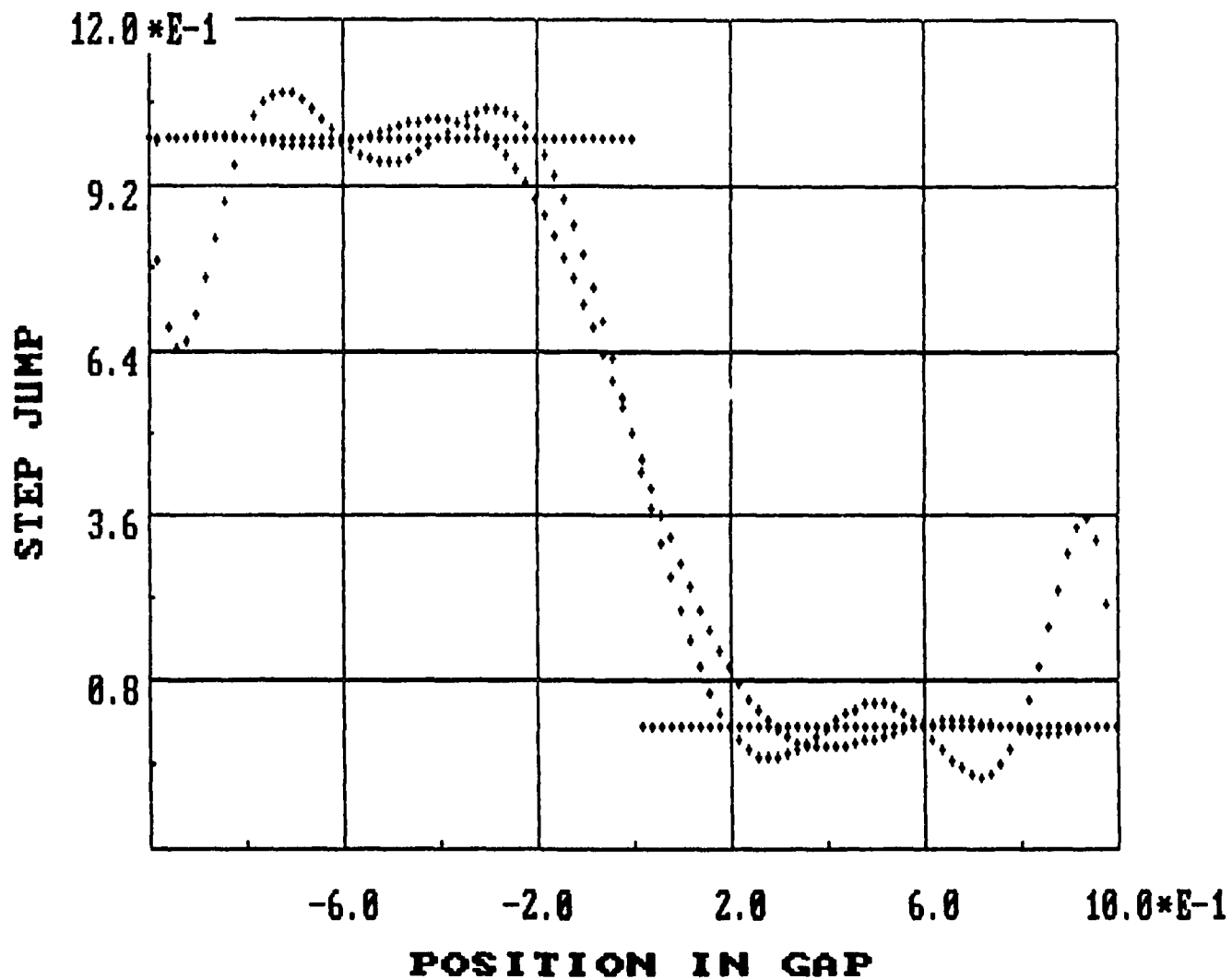
Figure 2. Representation of f(\xi) = (1 - \text{sgn}(\xi))/2 by 11 pt. Equidistant & Lobatto Interpolation
