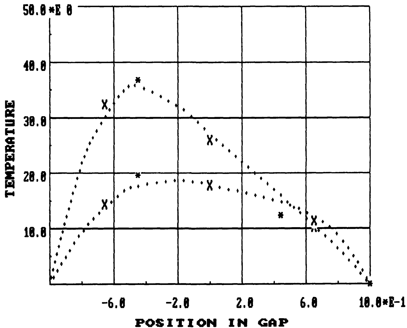
Figure 6. Temperature Profiles at Exit and Halfway Infinite-Width Slider, Variable Viscosity, h_1/h_2 = 2 N=8 (...); N=3 (*); N=2 (X)
