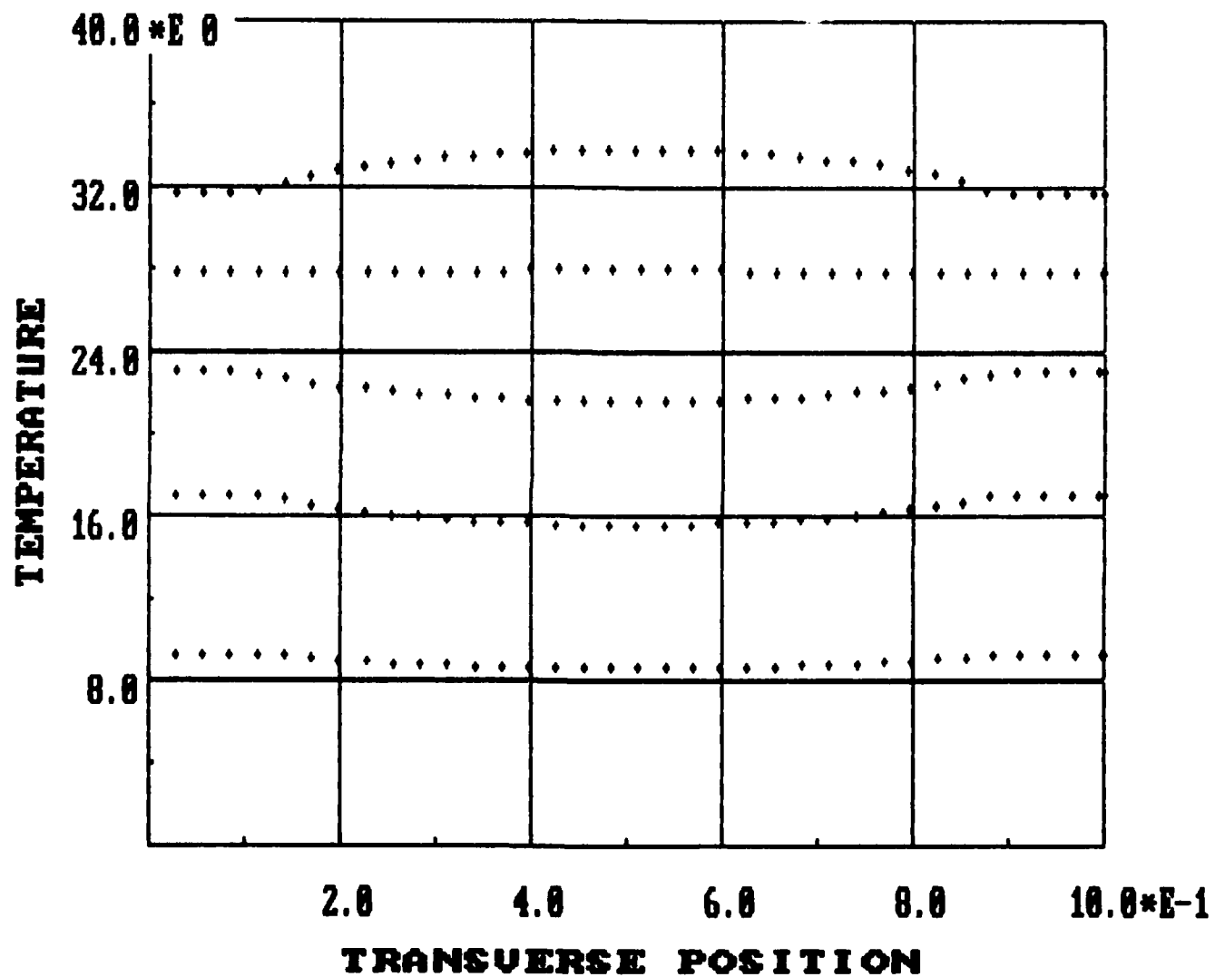
Figure 12. Temperature Profiles for Square Slider \zeta = -.657 , Variable Viscosity, h_2/h_1 = 2 N = 5
