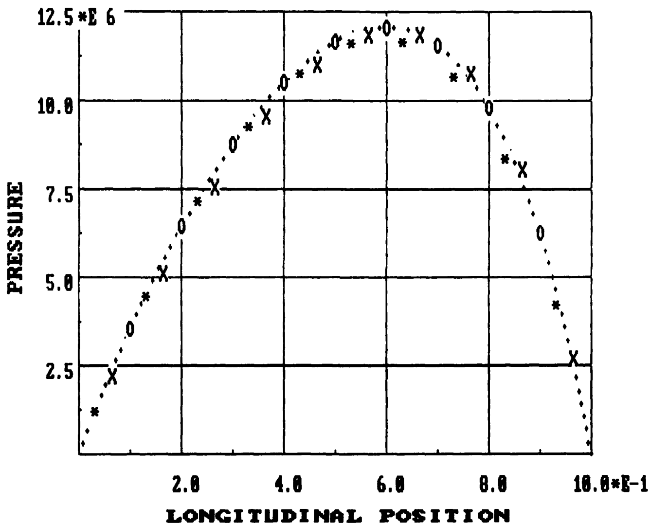
Figure 5. Convergence of Pressure Profiles with N Variable Viscosity, Infinite-Width Slider, h_1/h_2 = 2 N=8 (...); N=5 (O); N=3 (*); N=2 (X)
