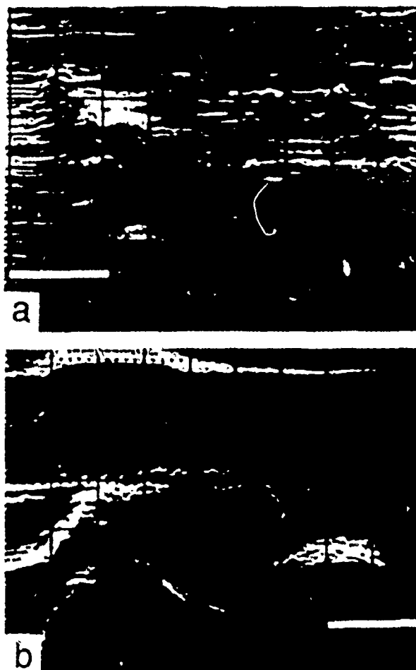
Figure 5. STM images of adsorbed lysozyme on HOPG, adsorption conditions: 0.1 mg/ml concentration, adsorption time 5 min at 22°C, and water rinse 1 min; STM conditions: constant height mode V_b = 800 mV, I_t = 2 nA. (a) Most lysozyme molecules merged into a rough adsorbed layer, bar = 40 Angstroms. (b) In very few cases globular molecules remained but their top portions were apparently truncated by the tip, bar = 40 Angstroms.
