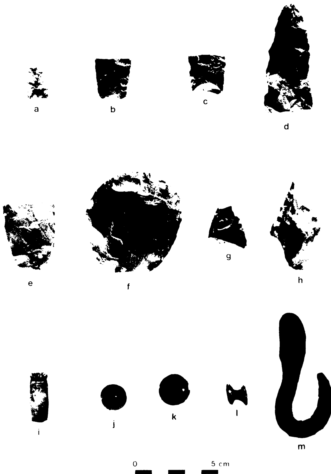
Figure 63. Artifacts from 23JA168, 23JA169, 23JA172 and 23JA173: (a) projectile point from 23JA168, (b-c) projectile points from 23JA169, (d-g) bifaces from 23JA169, (h) projectile point from 23JA172, (i-m) historic artifacts from 23JA173.
