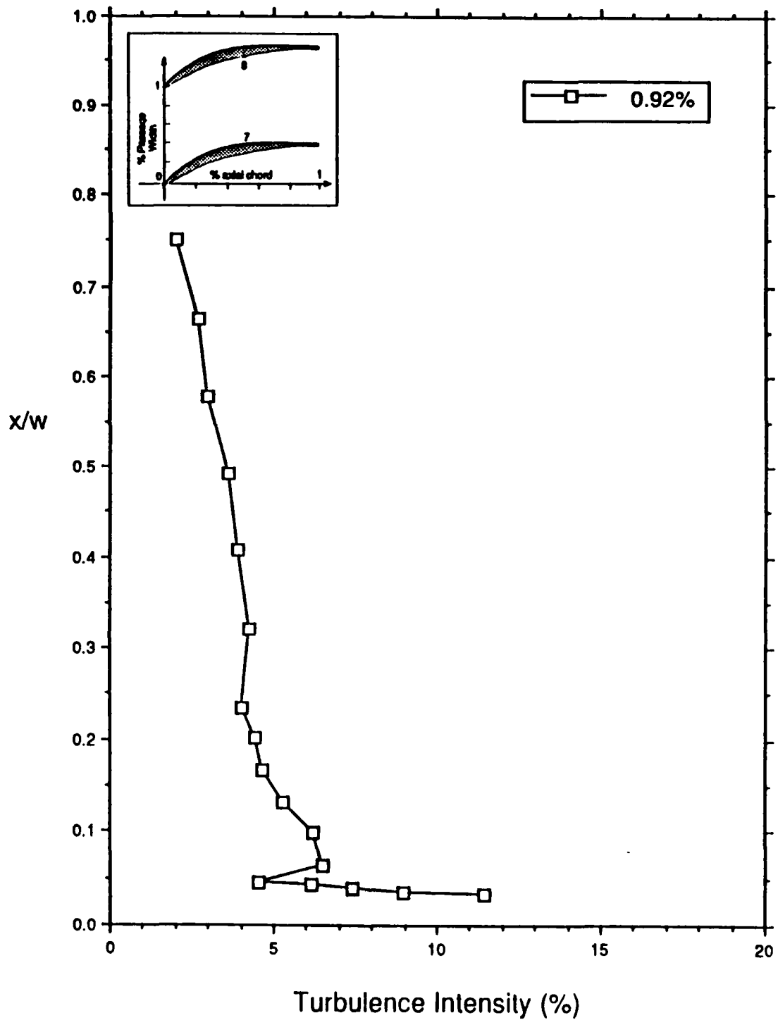
Figure 21. Passage Flow Survey: Turbulence Intensity Profile, 0.92% Axial Chord
