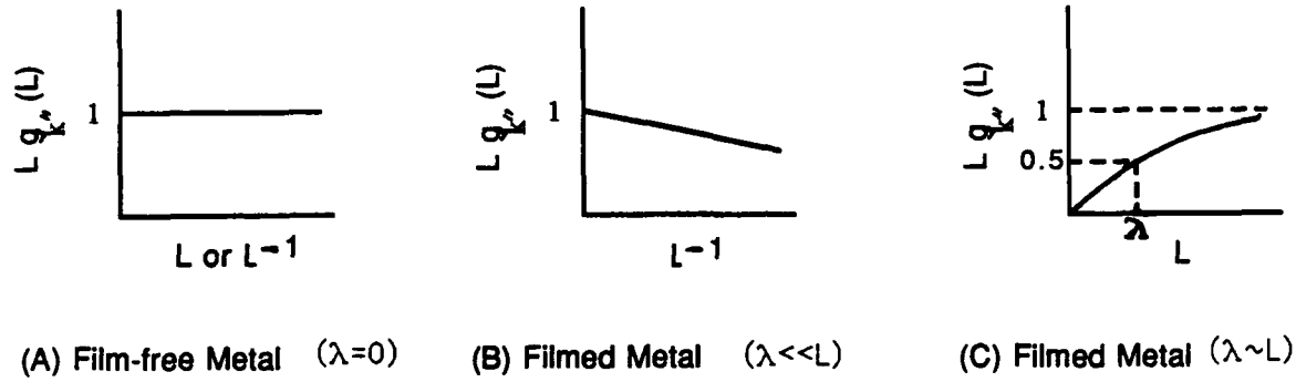
Figure 1: Schematic of film effect on L g_{k''}(L) versus L or L^{-1} plots.
