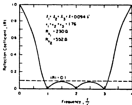
Normal-incidence reflection coefficient of a three-layer Salisbury screen versus frequency.
