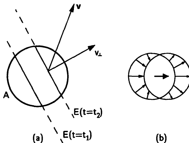
Figure 7: An illustration of the aperture problem. Left: a bar E is moving behind a small aperture A , so that its ends are not visible. Only the component v_{\perp} of the bar's velocity that is perpendicular to the bar's orientation can be measured through the aperture. Right: an example of a circle translating to the right. The component perpendicular to the circle's contour, which would be computed by aperture-limited operators, does not correspond to the true motion of the circle.
