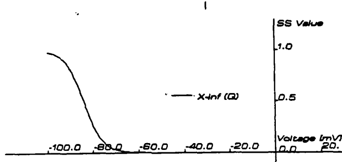
Figure 7.27: Steady-state curve ( x_\infty ) for x_Q .
