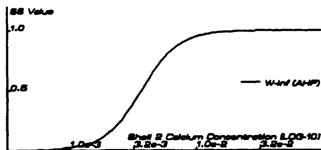
Figure 7.22: Relation between u_x and [Ca^{2+}]_{\text{shell},2} for w_{AHP} .
