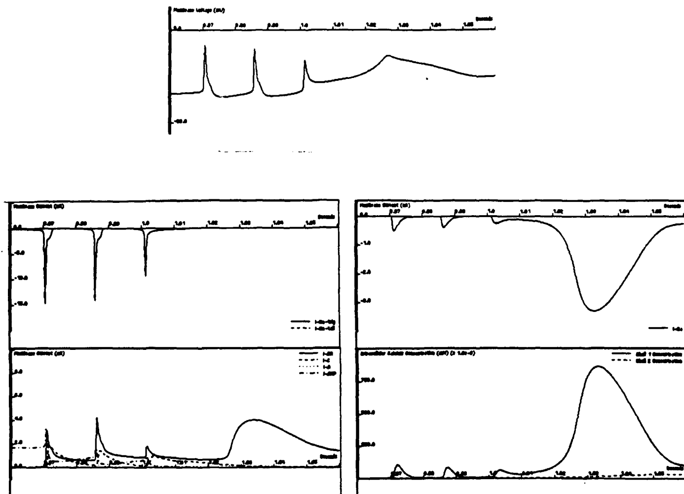
Figure 9.16: Degeneration of spike train without I_{Na-rep} - Soma response. Na^+ currents, K^+ currents, I_{Ca} , and intracellular Ca^{2+} concentrations. Note the eventual strong activation of I_{Ca} preceding stable depolarization.
