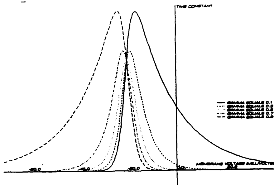
Figure 4.7: Effect of the relative position, \gamma , of the transition state within the membrane for the gating particle, x , on the \tau_x curve. z = 16 and V_1 = -20mV . The time scale is arbitrary, as in Figure x. \tau_0 is set to 0.
