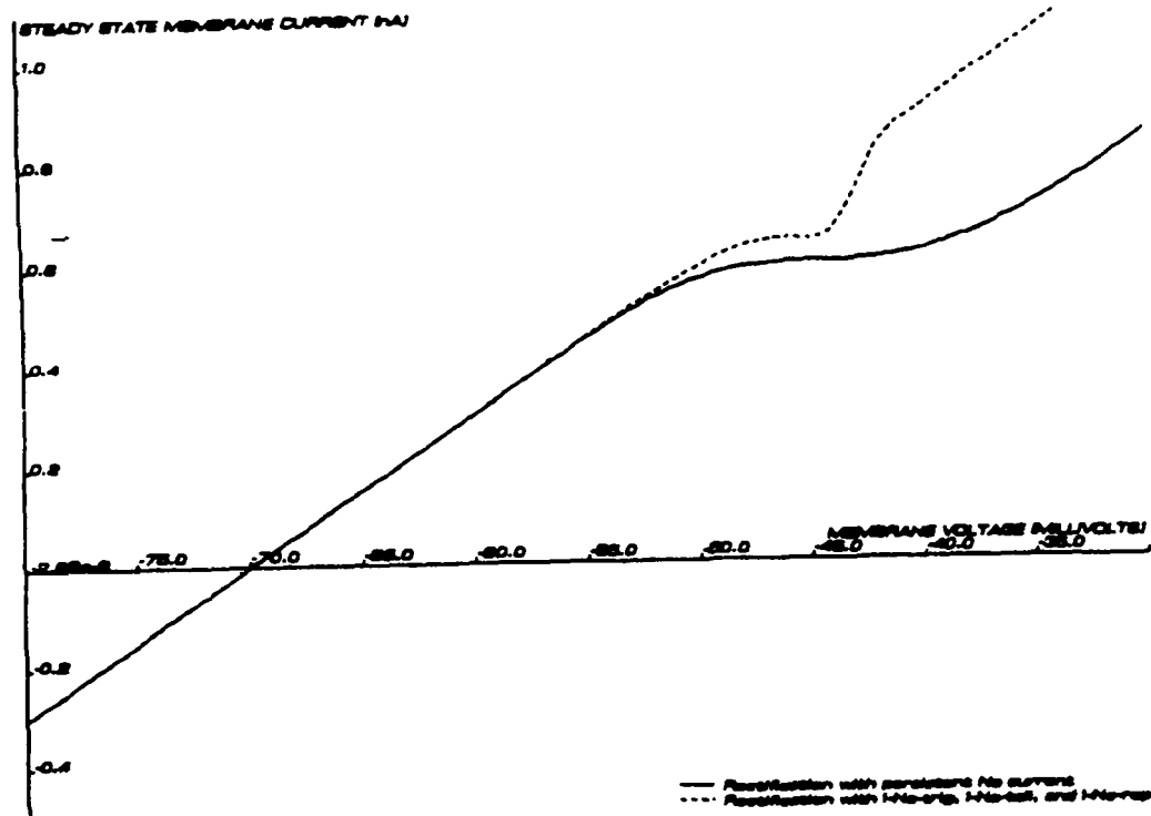
Figure 5.5: Current-voltage characteristics of model showing inward-rectification mediated by I_{NaP} and by I_{Na-trig} , I_{Na-tail} , and I_{Na-rep} currents.
