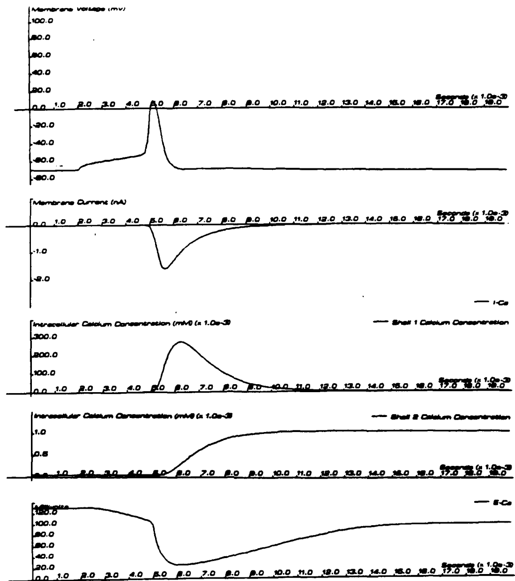
Figure 6.8: Top - Simulation of normal action potential. Top Middle - I_{Ca} during spike. Bottom Middle - [Ca^{2+}]_{shell.1} during spike. Bottom - E_{Ca} during spike.
