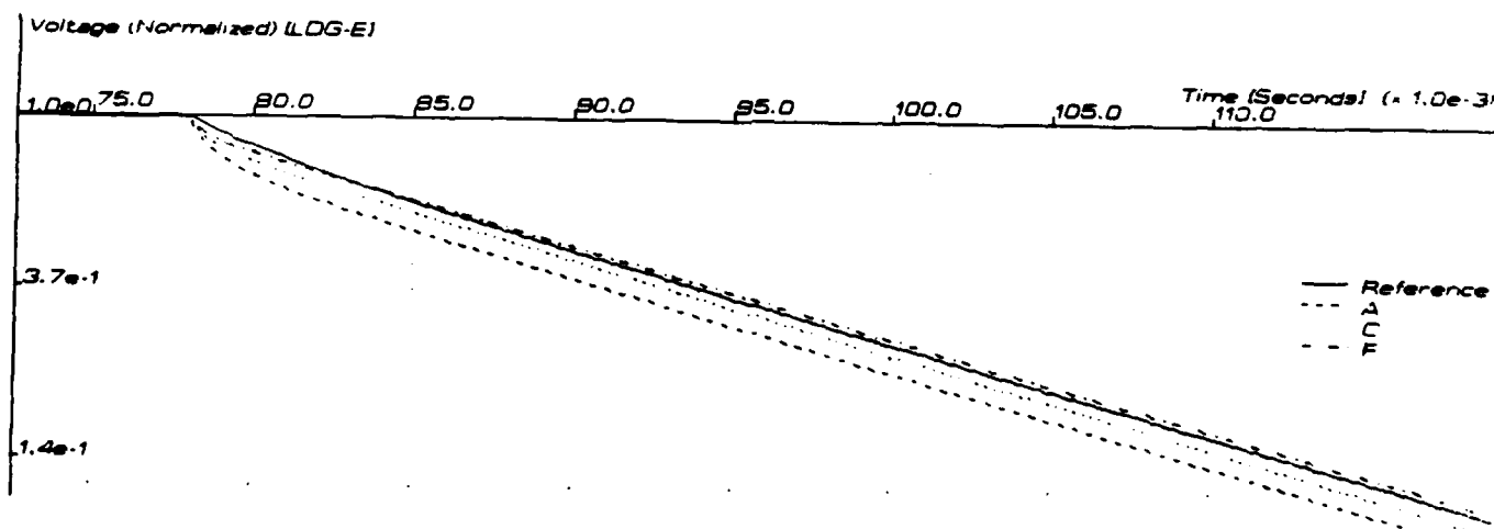
Figure 3.11: Semi-log plot of Figure 3.9, showing the rapid approach to a single exponential decay ( \tau_0 = 19 ms) for all the structures.
