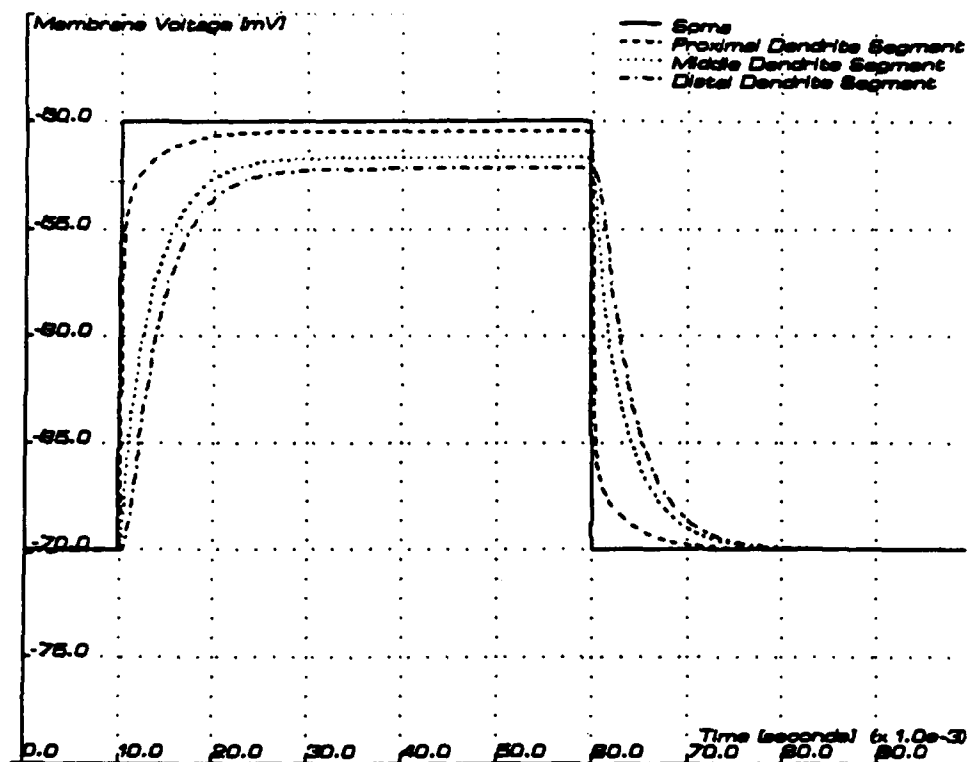
Figure 8.1: Voltage clamp simulation with clamp applied to the soma. The voltage step seen by the different parts of the dendrite membrane is distorted.
