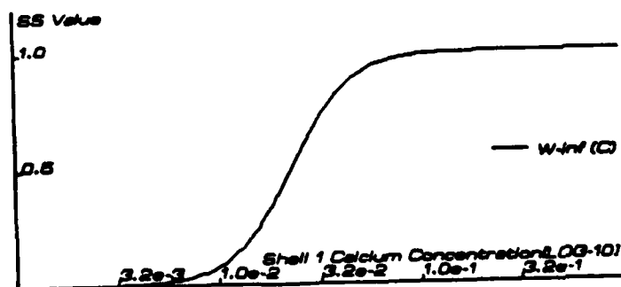
Figure 7.15: Relation between u_{\infty} and [Ca^{2+}]_{\text{shell}} for u_C .
