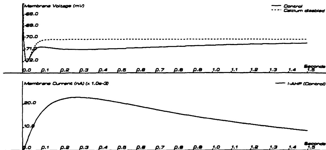
Figure 7.17: Top - Repolarization of the action potential with and without \text{Ca}^{2+} blockers (Storm). Note absence of sAHP when \text{Ca}^{2+} blockers are added. Bottom - Simulation of protocol.
