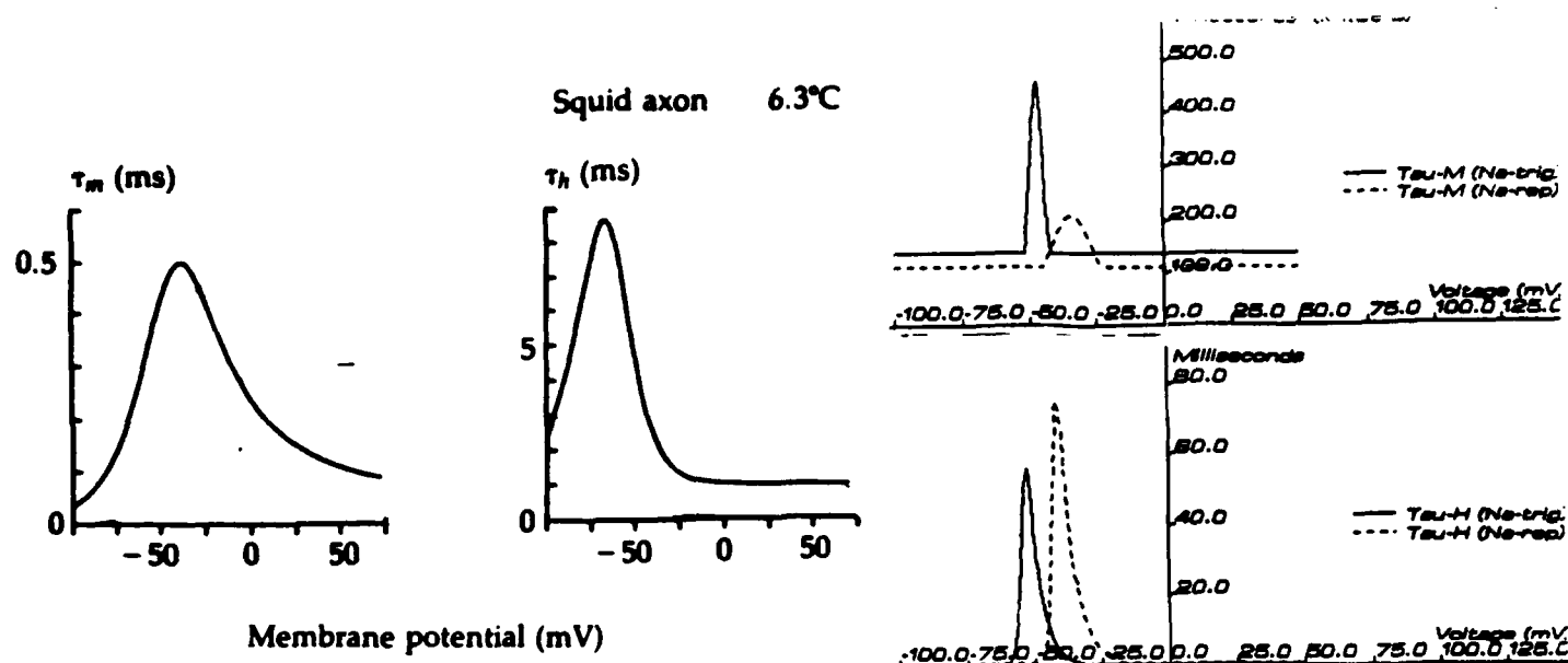
Figure 5.16: Time constant curves ( \tau_m and \tau_h ) for squid axon I_{Na} and the hippocampal I_{Na-trig} and I_{Na-rep} .
