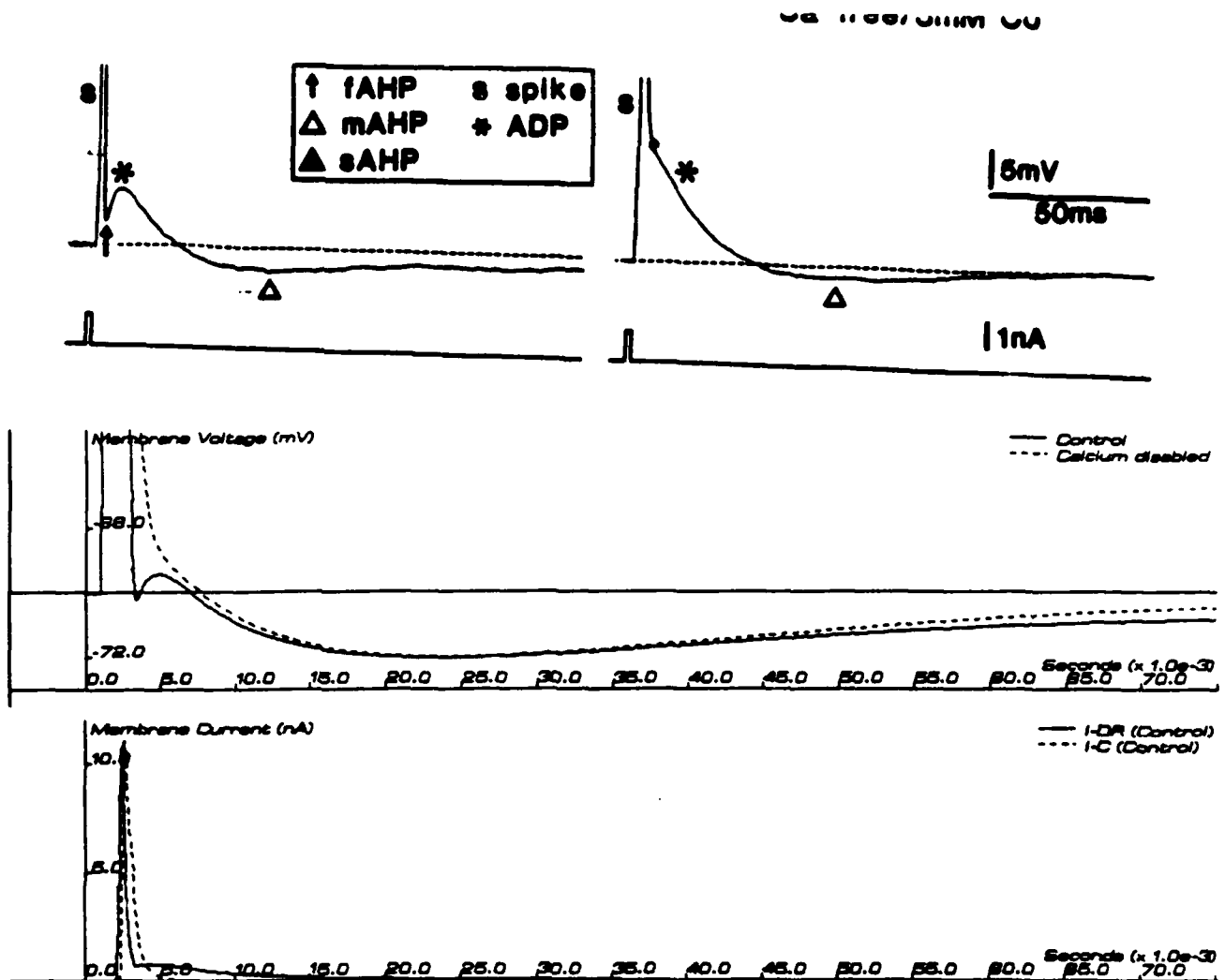
Figure 7.11: Top - Repolarization of the action potential with and without Ca^{2+} blockers (Storm, 1986b). Note absence of fAHP when Ca^{2+} blockers are added. Bottom - Simulation of protocol.
