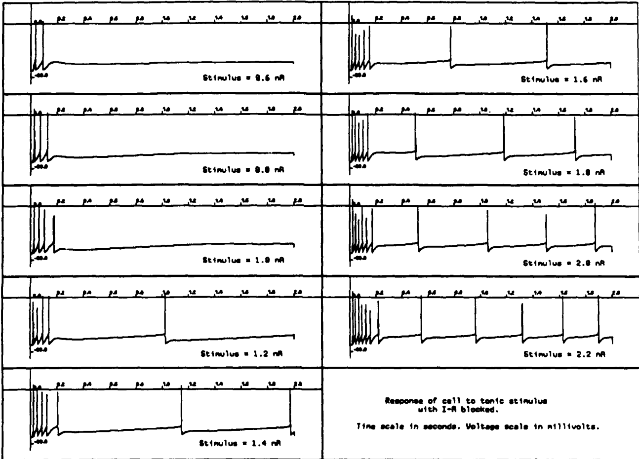
Figure 9.2: Simulations of response to tonic somatic input with I_A disabled. Stimulus strengths include 0.6 nA, 0.8 nA, 1.0 nA, 1.2 nA, 1.4 nA, 1.6 nA, 1.8 nA, 2.0 nA, and 2.2 nA.
