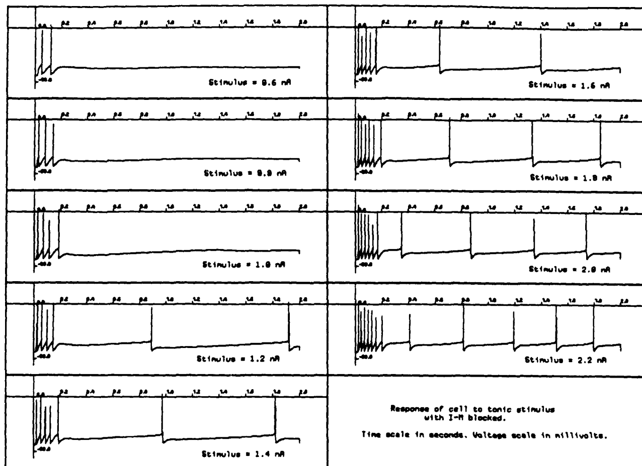
Figure 9.3: Simulations of response to tonic somatic input with I_M disabled. Stimulus strengths include 0.6 nA, 0.8 nA, 1.0 nA, 1.2 nA, 1.4 nA, 1.6 nA, 1.8 nA, 2.0 nA, and 2.2 nA.
