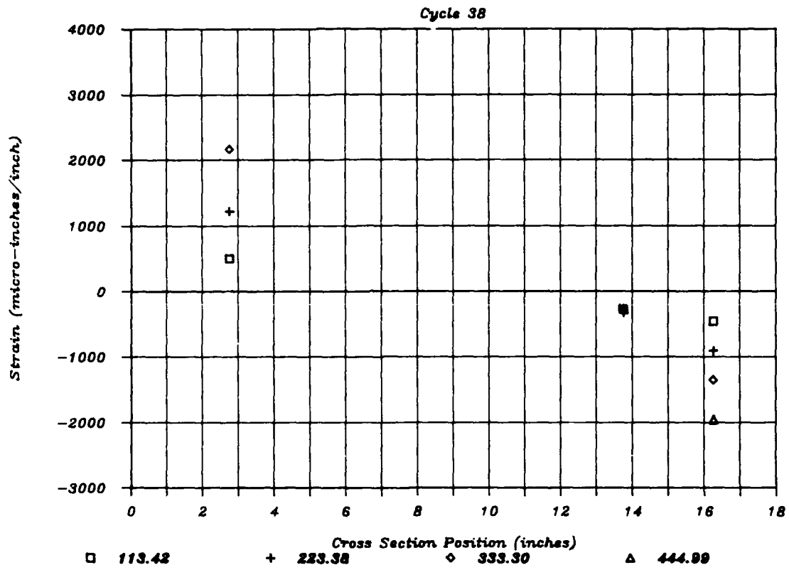
Figure B-1. MK1 load point cross-section strain - final cycle.
