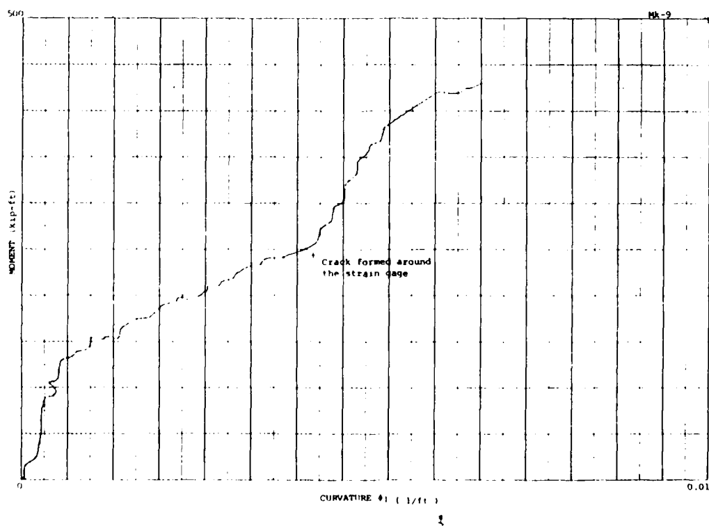
Figure B-119. MK9 moment-curvature plot.
