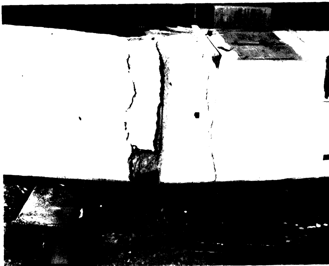
Figure B-4. MK1 post-failure tensile cracking at the load point.
