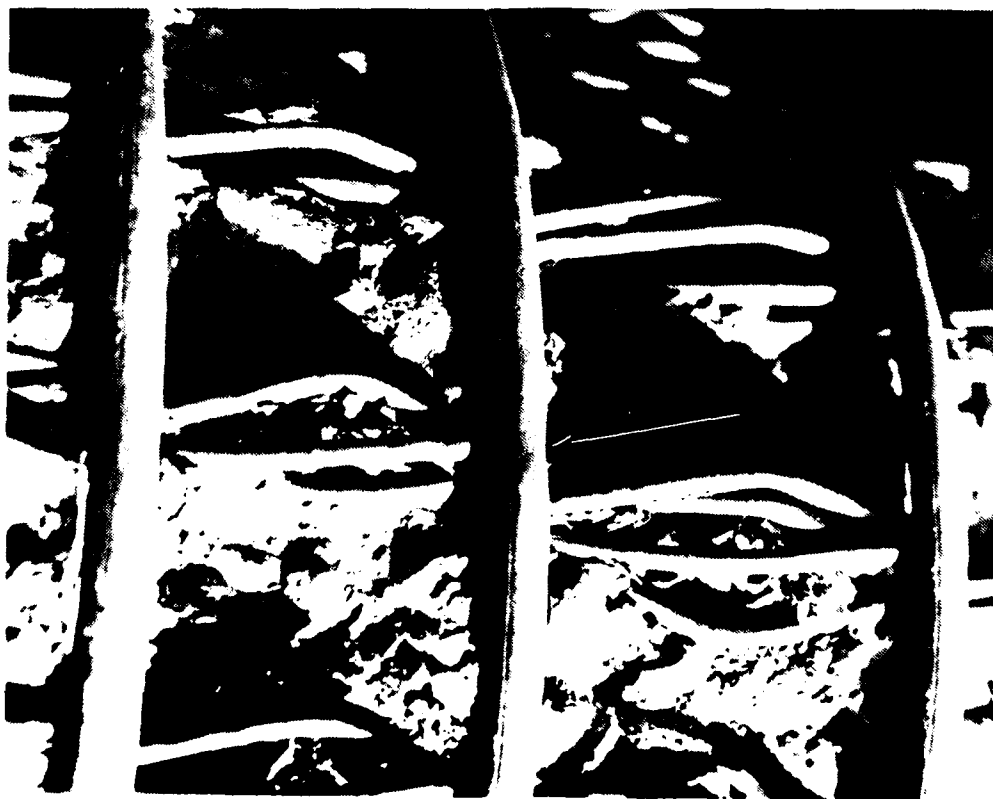
Figure B-81. MK7 spiral yield and necking in the spall zone.
