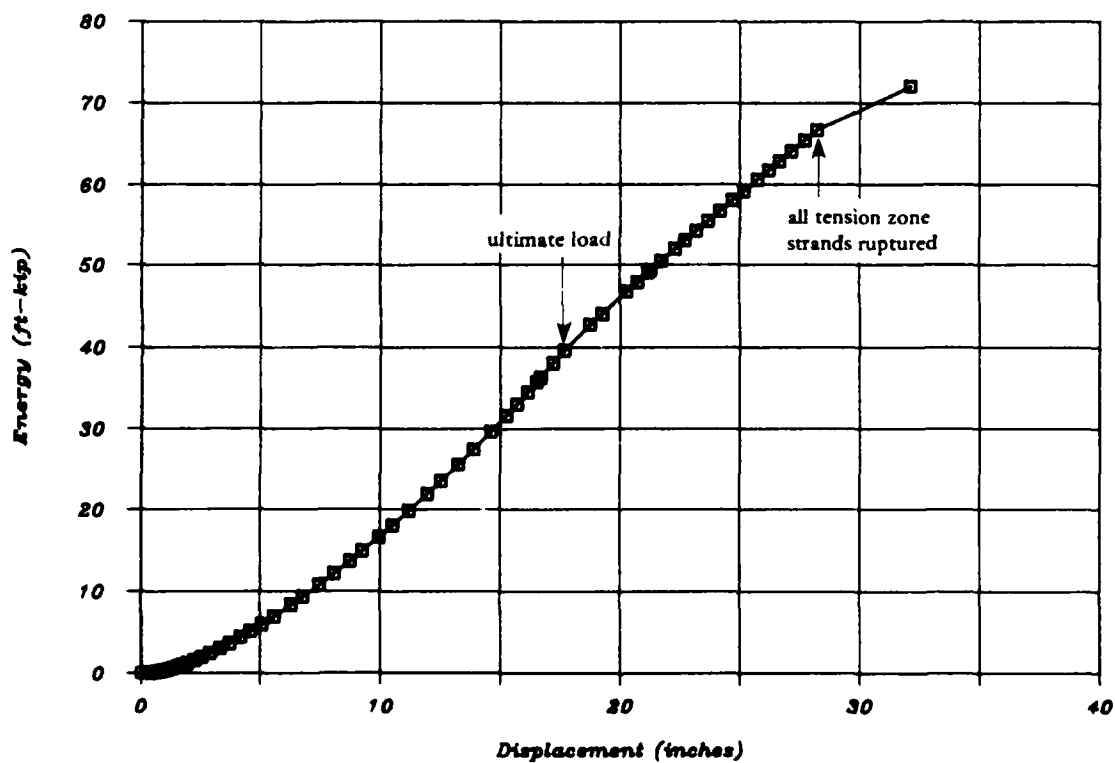
Figure B-75. MK6 energy-displacement plot.
