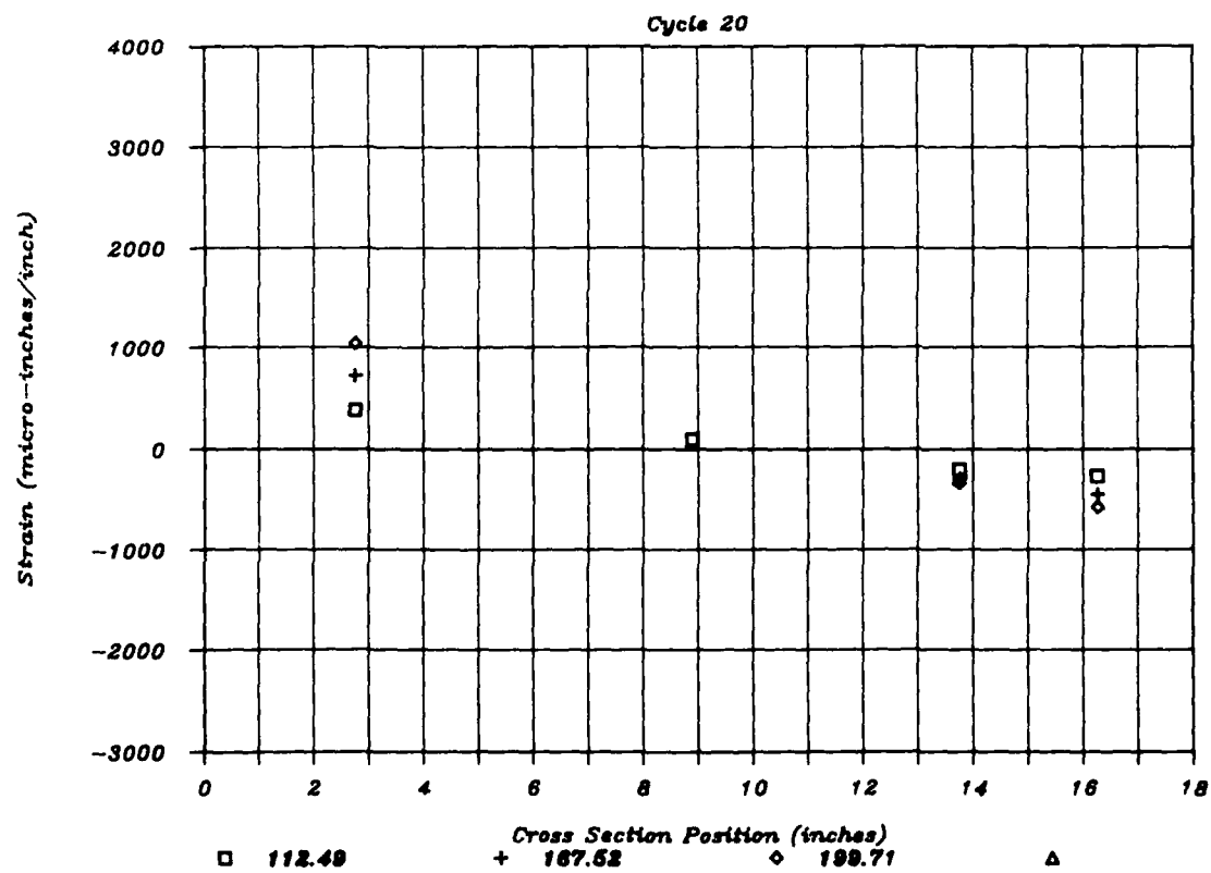
Figure B-18. MK1 load point cross-section strain - cycle 20.
