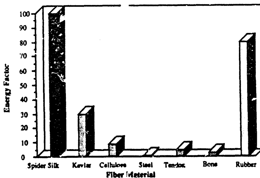
GRAPH 3: Relative Energy Absorption To Break Fiber Materials
