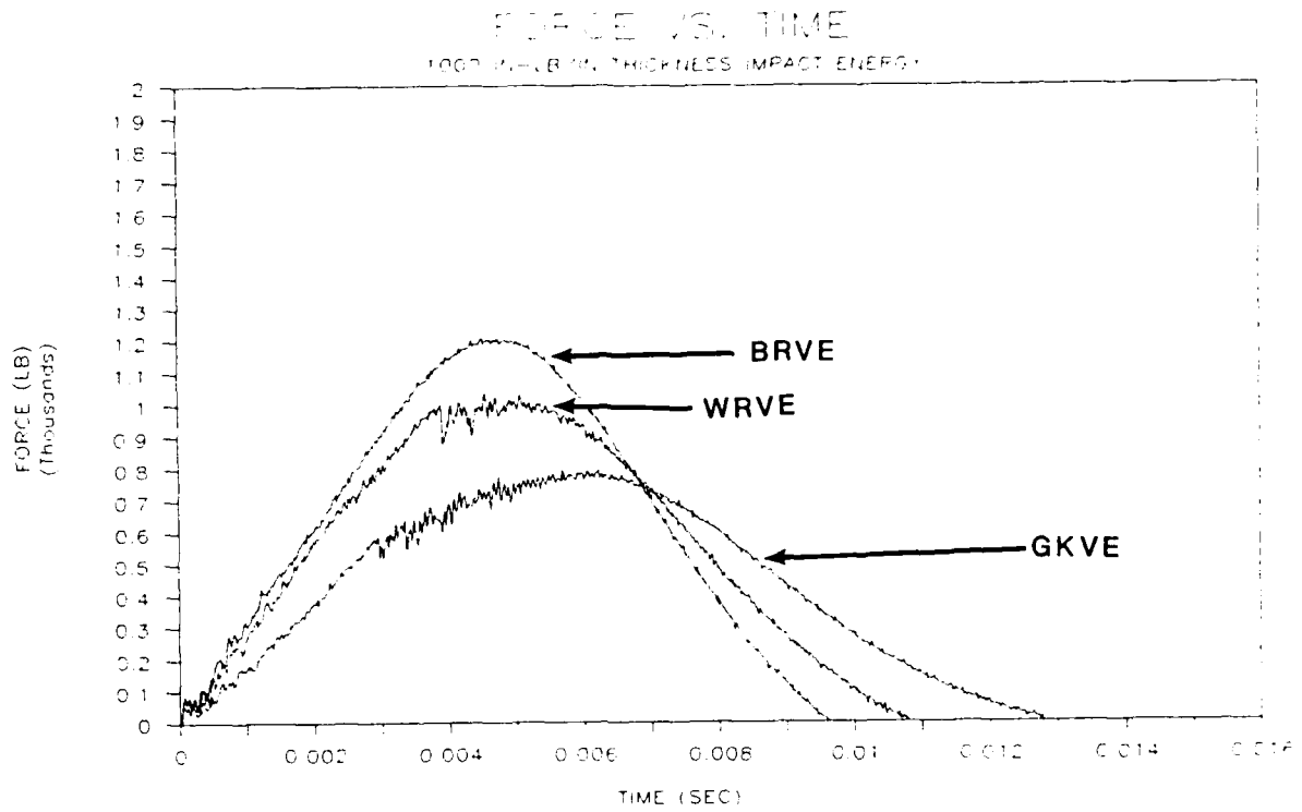
Fig. 18 Force-time curves for WR/VE, BR/VE, and GK/VE impacted at 1000 in. lbs./in. with the 0.5 in. diameter tup
