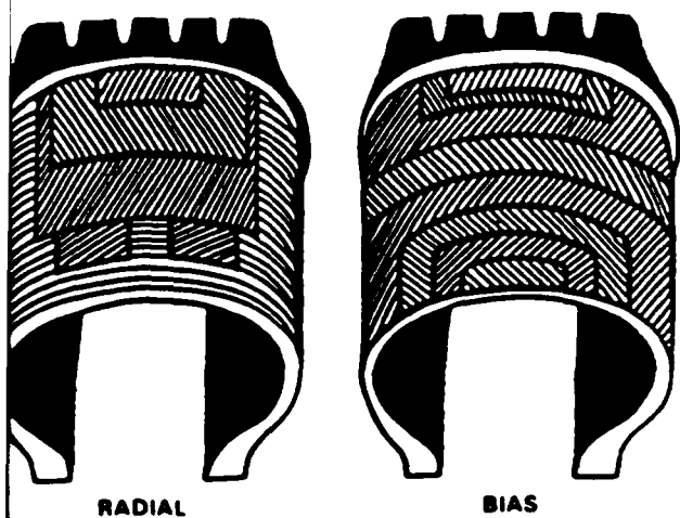
Radial v. Bias Construction
