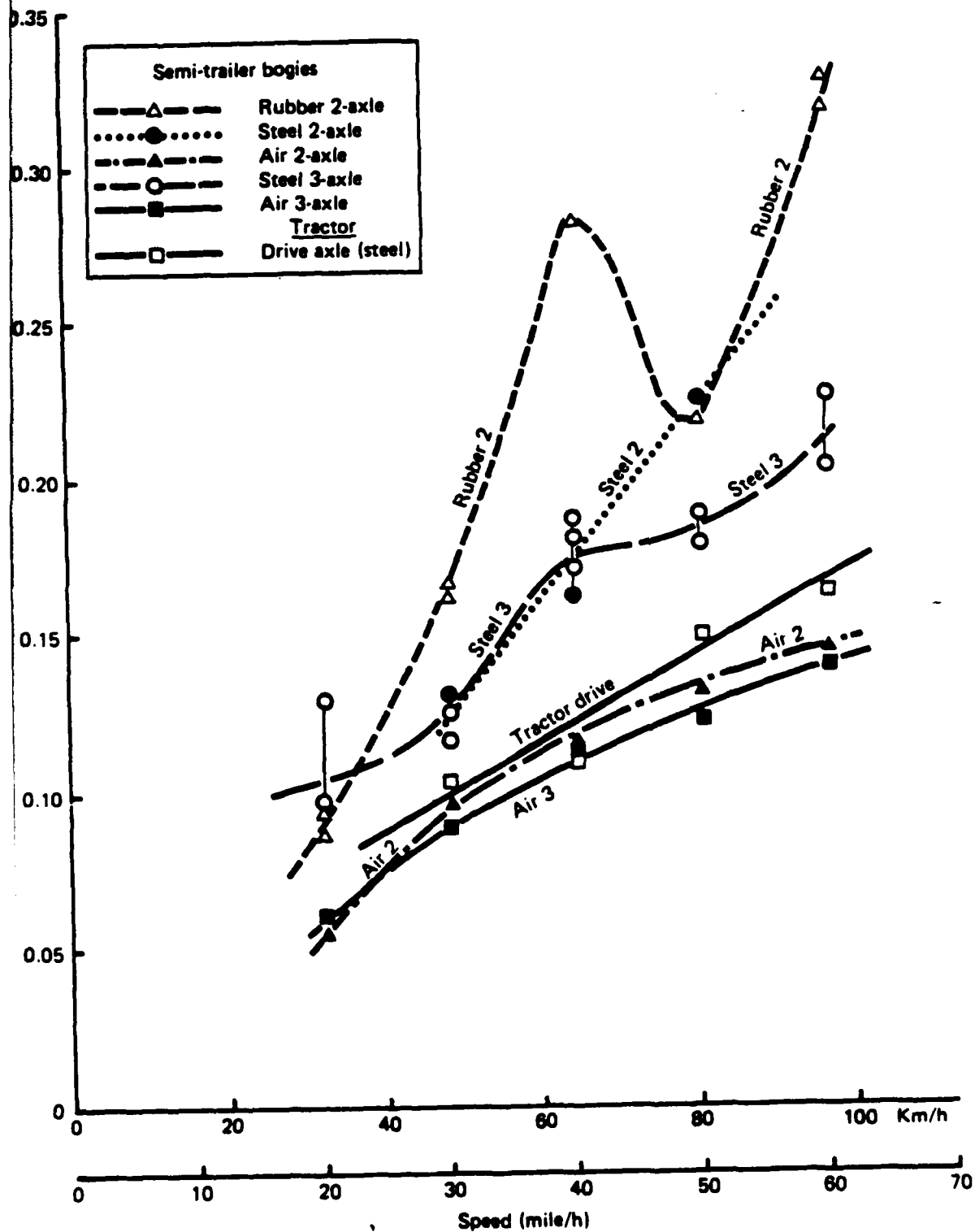
Dynamic load coefficients for the tractor drive axle and 2- and 3- axle semi-trailer bogies on the rough section of the TRRL track. Vehicles fully loaded
