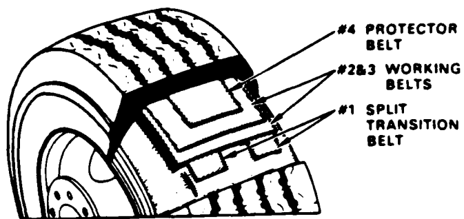
Typical Radial Construction
