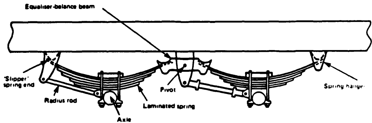
Leaf Spring
