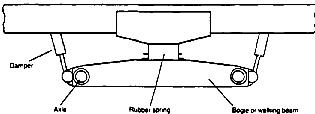
Walking Beam
