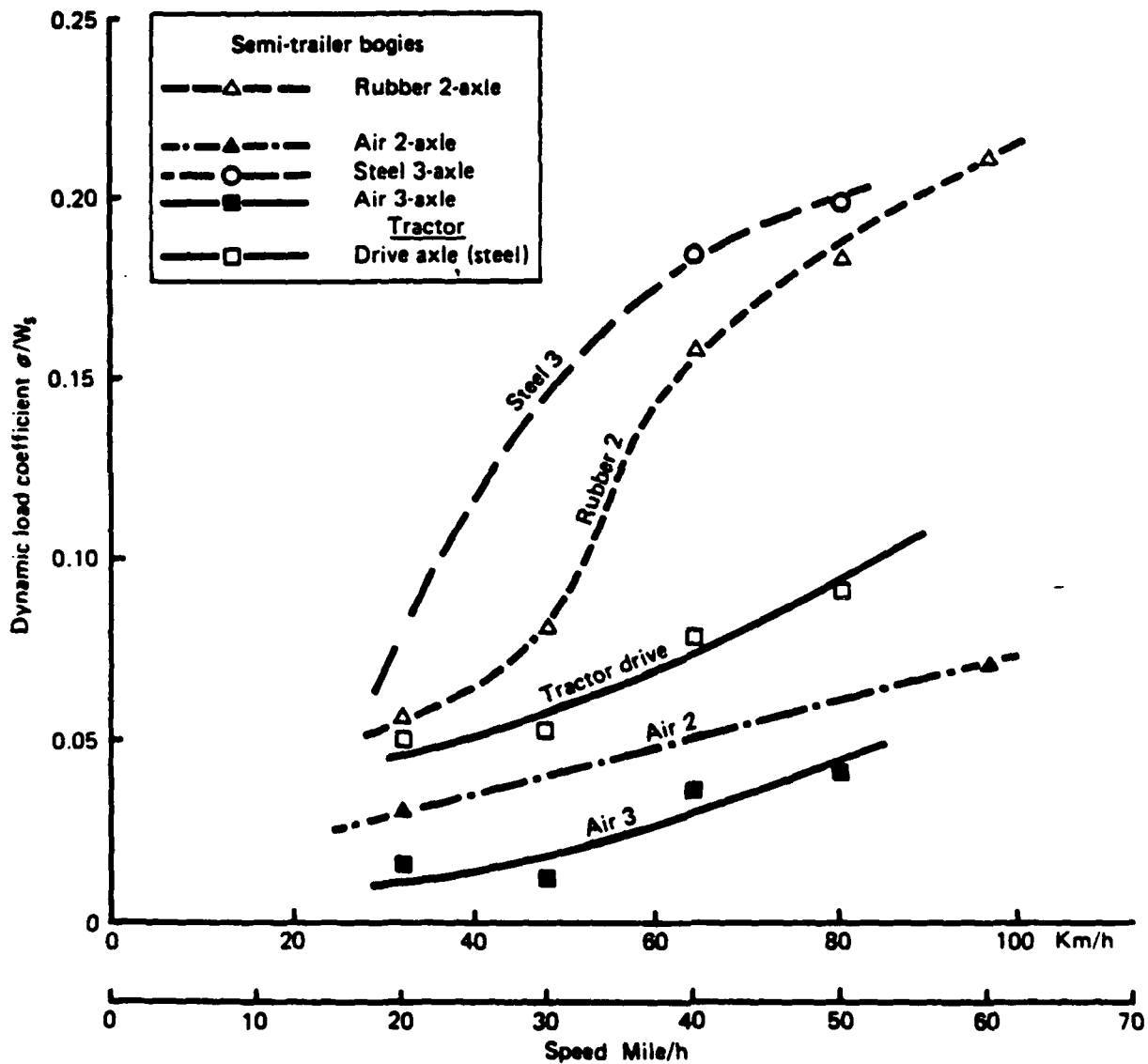
Dynamic load coefficients for the tractor drive axle and 2-and 3-axle semi-trailer bogies on the smooth section of the TRRL track. Vehicles fully loaded
