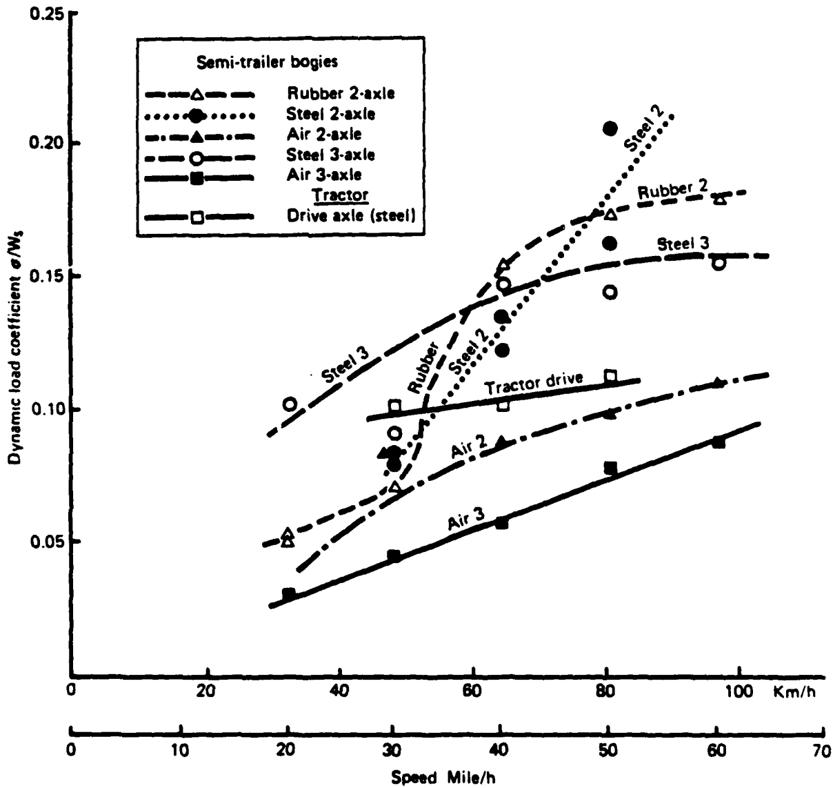
Dynamic load coefficients for the tractor drive axle and 2-and 3-axle semi-trailer bogies on the medium section of the TRRL track. Vehicles fully loaded
