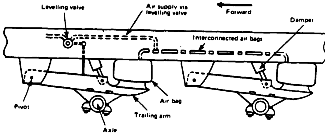
Air Cushion
