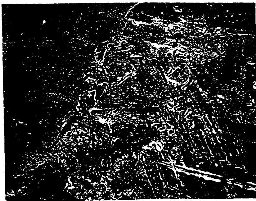
FIGURE 16: HASTELLOY G30 - 2 DAY EXPOSURE TO BrF 3 ~600X
