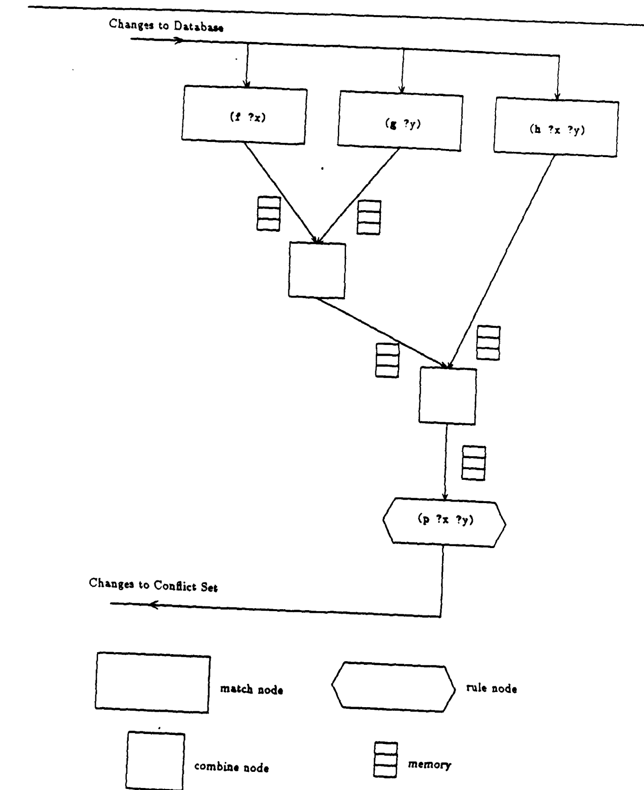
Figure 2-2: A Rete Network.
