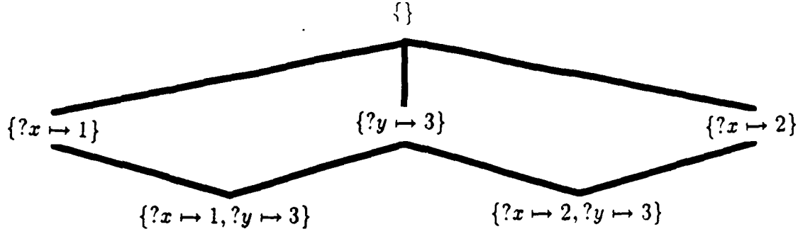
Figure 3-2: Semi-Lattice of Substitutions.
