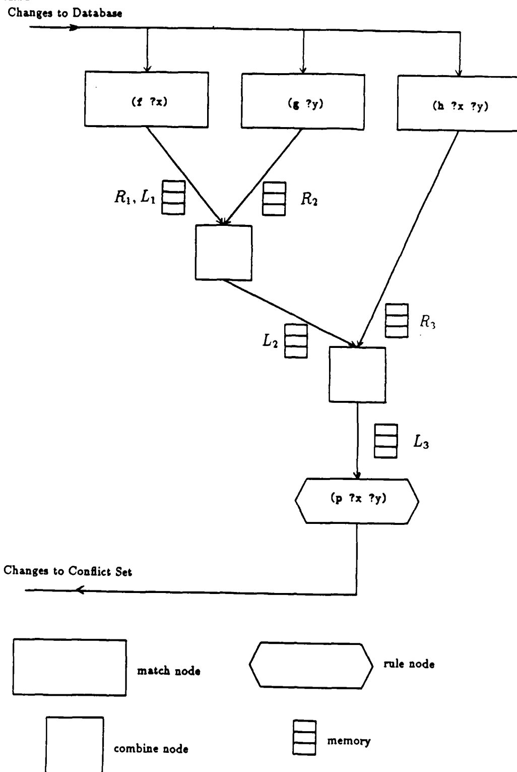
Figure 4-2: Correspondence between Match-Rule and the Rete Network.
