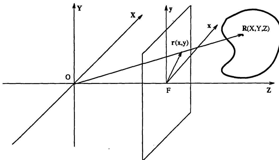
Figure 2.1: Perspective transformation
