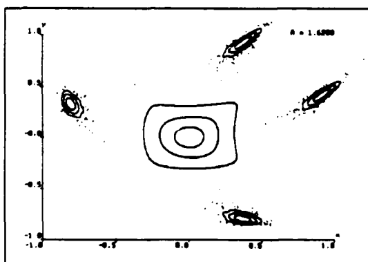
(c) The 4-island chain becomes unbounded.
