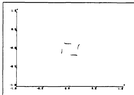
(a) First 128 iterates
