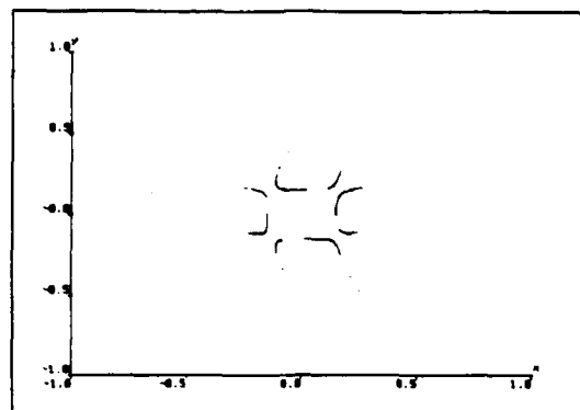
(a) First 384 iterates
