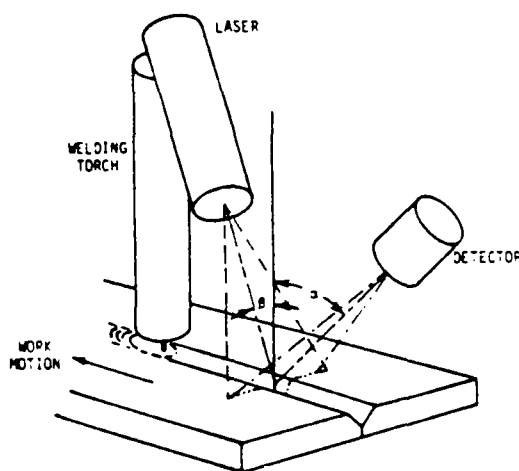
Figure 2.14 Typical optical sensor configuration. (55)
