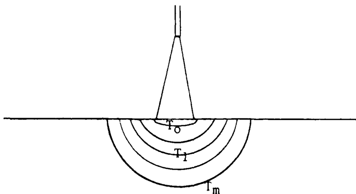
Figure 3.1 Isotherm patterns in a purely conductive weld pool. T_o > T_1 > T_m
