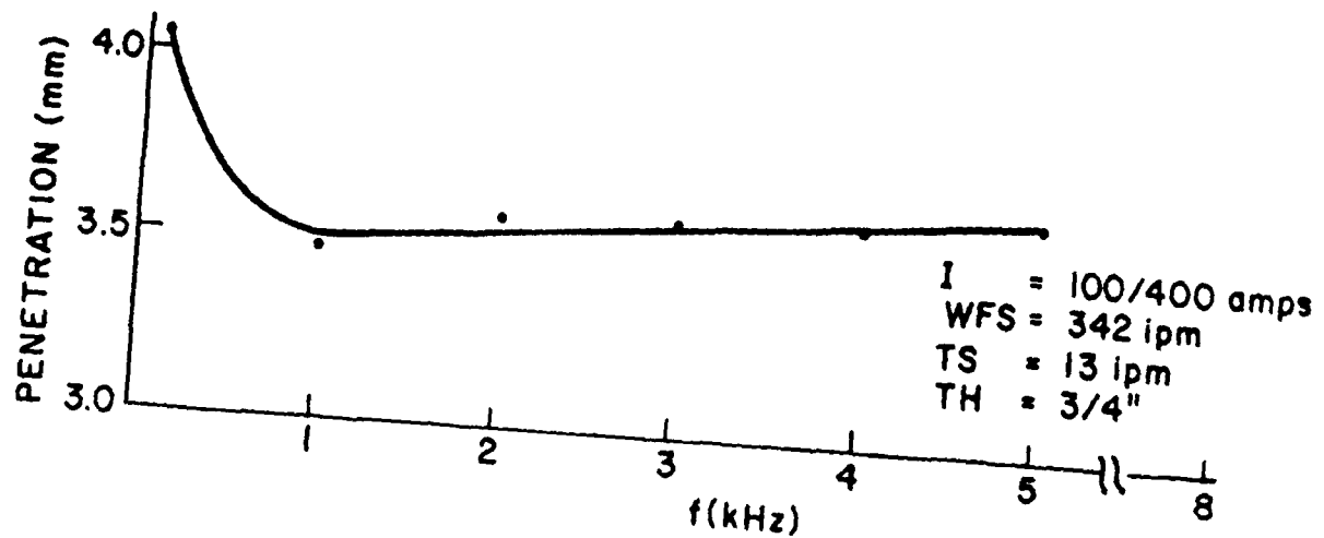
Figure 6.10 Penetration at high frequencies, data set #1.
