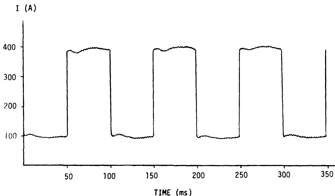
Figure 5.1 Current regulator output waveform.
