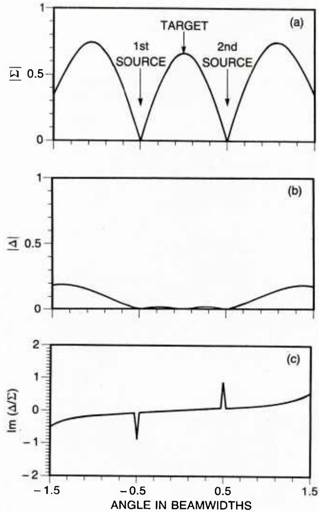
Fig. 4 — Two interference sources at 0.5 and -0.5 beamwidth, respectively: (a) sum pattern; (b) difference pattern; (c) monopulse error curve
