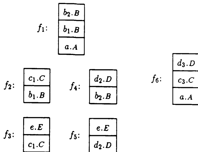
Figure 9.1: Logs generating non-optimal estimates
