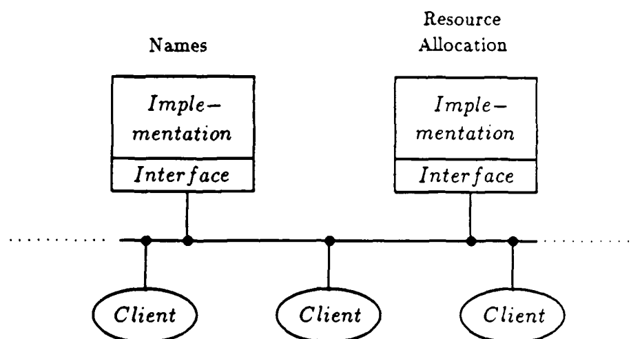
Figure 1.1: An object-oriented system
