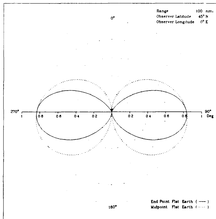
Fig. 4 — Flat Earth bearing errors vs azimuth
