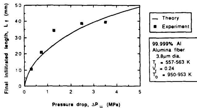
Fig. 11—Effect of pressure drop on final infiltrated length. Calculations assume h_c = 200 \text{ W/m}^2 \text{ K} .
