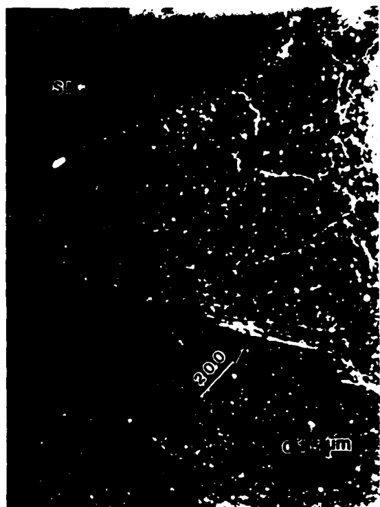
Fig. 9. g_{3g} weak beam dark field image of an area in the aluminum matrix near the aluminum-SiC interface.
