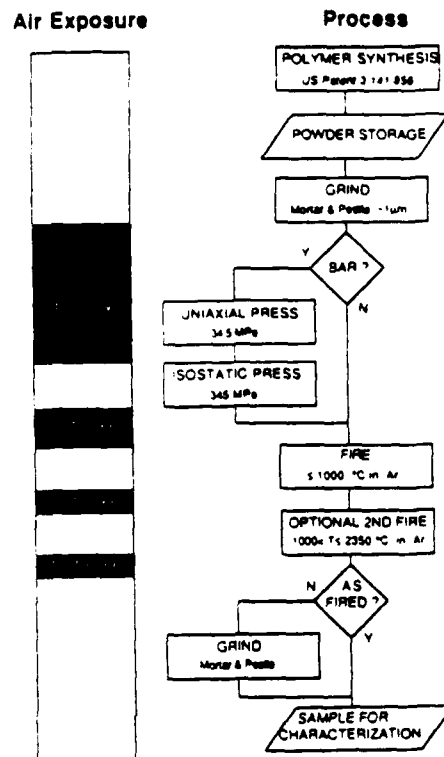
Fig. 1 Summary of processing steps used to make B_4C ceramic from POP polymer precursor. Occurrences and durations of exposure to air are shown.
