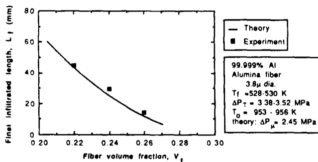
Fig. 12—Effect of fiber volume fraction on final infiltrated length. Theoretical curve assumes h_c = 200 \text{ W/m}^2 \text{ K} .
