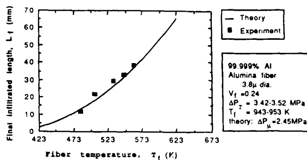
Fig. 13—Effect of fiber temperature on final infiltrated length. Theoretical curve assumes h_c = 200 \text{ W/m}^2 \text{ K} .
