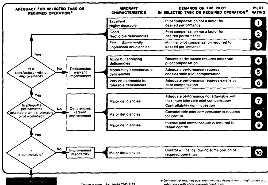
Figure 10.— The Handling-Qualities Rating Scale.
