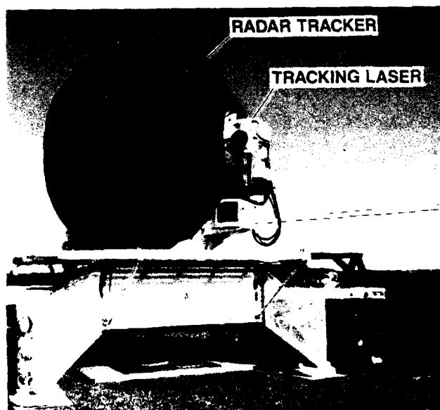
Figure 11.— Laser tracker.
