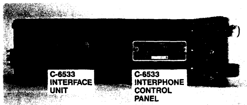
Figure 7.— Interface box.
