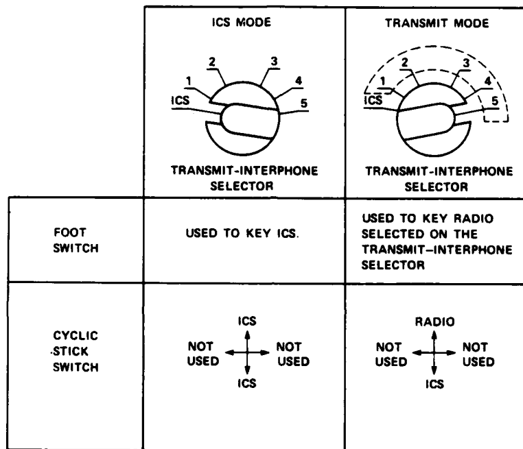
Figure B-1.— Original configuration.
