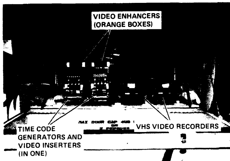
Figure 13.— Time-code generators and video support equipment; view 1.
