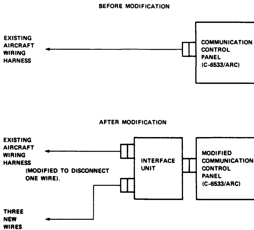
Figure C-1.— Modification of communication system for design option 5.
