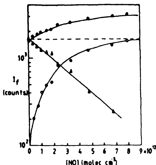
FIG. 7. Variation with NO number density in the afterglow [NO] of the LIF intensity from OH I_f (photon counts per 250 laser shots, filled circles) for the R_1(1) line in the A^2\Sigma(\nu = 1) - X^2\Pi(\nu' = 0) excitation spectrum (see Fig. 3). OH X^2\Pi(\nu' > 0) and X^2\Pi(\nu' = 0) were produced upstream of the NO addition point from the dissociative recombination of \text{HCO}_3^+ . The increase in I_f with [NO] is due to quenching of OH( \nu' > 0 ) by NO to produce OH( \nu' = 0 ) [reaction (21)]. Thus the change in I_f between zero [NO] and the asymptotic value at large [NO], relative to the value of I_f at zero [NO], represents the amount of OH( \nu' > 0 ) relative to OH( \nu' = 0 ) which is produced in the \text{HCO}_3^+ recombination reaction. The increase in OH( \nu' > 0 ) can be seen more clearly (open circles) by subtracting the contribution of OH( \nu' = 0 ) from I_f . The effective rate coefficient for the quenching reaction can be deduced from the slope of the linear plot (triangles) which was obtained by subtracting the values represented by the open circles from the asymptotic value at large [NO], as represented by the dashed line.
