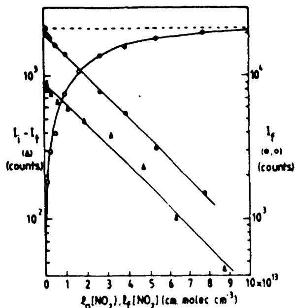
FIG. 4. Decrease in the absorption L_i - I_f (counts per 50 s) of L_\alpha radiation by H atoms (triangles) as a function of the product l_f [\text{NO}_2] due to the calibration reaction \text{H} + \text{NO}_2 \rightarrow \text{OH} + \text{NO} [reaction (2)]. [\text{NO}_2] is the number density of \text{NO}_2 molecules introduced into the afterglow at port I4 and l_f is the reaction length between this port and the position at which the H atoms are monitored (see Fig. 1). Also given is the related increase in the LIF intensity of OH I_f (open circles) (fluorescence photon counts per 500 laser shots) for the P_1(5) line in the A^2\Sigma(\nu=1) - X^2\Pi(\nu''=0) excitation spectrum (see Fig. 3) with increasing l_f [\text{NO}_2] where l_f is the reaction length between port I4 and the laser beam. Both l_i and l_f are included since these reaction lengths for H atom and OH radical detection are different (35.5 and 17.5 cm, respectively). The filled circles were obtained by subtracting the OH fluorescence intensities from the asymptotic value at large l_f [\text{NO}_2] (as given by the dashed line). This line and that for the L_\alpha absorption give values of the rate coefficient for the \text{H} + \text{NO}_2 reaction which are in good agreement with the literature value (see the text).
