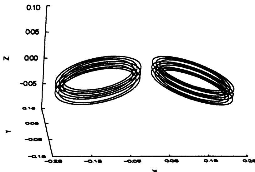
Figure 2. Initial vortex ring configuration.
