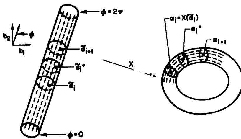
Figure 1. Discrete parameterization of a vortex ring.
