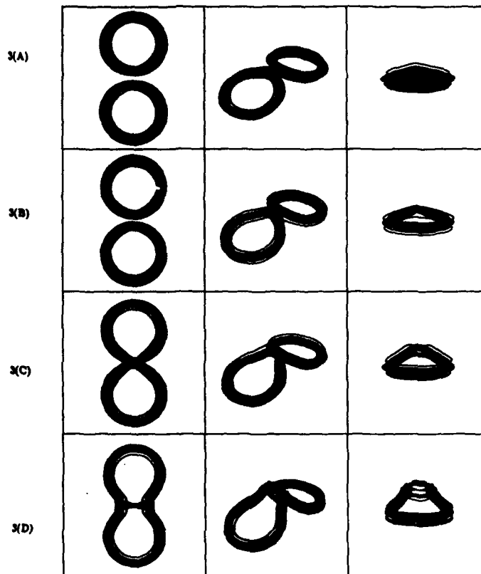
Figure 3. Perspective Views of Vortex Rings. Rows (A)–(D) are the vortex ring configurations at steps 16, 32, 48, and 64, with time steps of size .25 \times 10^{-4} , second-order Runge-Kutta time integration, and \delta = .012 . The first column is a top view of the rings; the view is along the z -axis. The second column is a corner view of the rings, along the vector (1, 1, \frac{1}{2}) . The third column is a view along the x -axis; the far ring is deleted from the plot for the sake of clarity.
