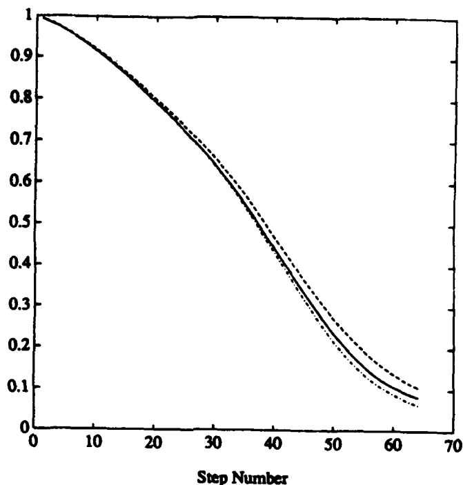
Figure 7. ----: relative core distance \epsilon = .015 ; —: relative core distance \epsilon = .012 ; ....: relative core distance \epsilon = .010 .
