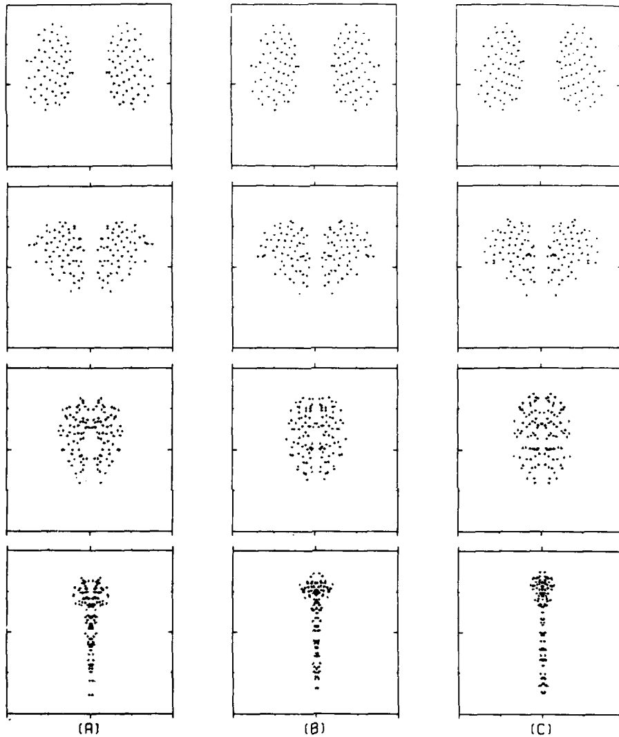
Figure 6. Vortex core cross-sections. (A): \epsilon = .015 , Steps 16, 32, 48, 64; (B): \epsilon = .012 , Steps 16, 32, 48, 64; (C): \epsilon = .010 , Steps 16, 32, 48, 64.
