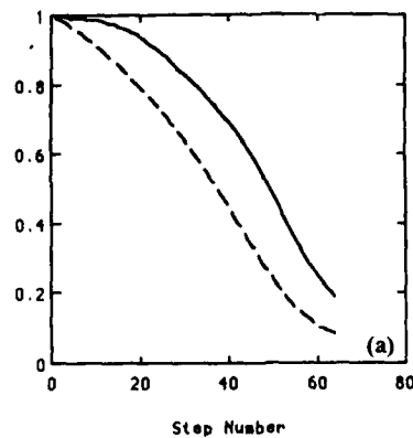
Figure 5(a). —: relative x location of vortex core; ----: relative core cross-sectional area.
