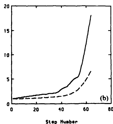
Figure 5(b). —: Maximum relative stretching; ----: average relative stretching.
