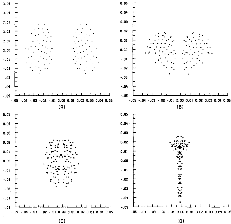
Figure 4. Vortex core cross-sections. (A)-Step 16; (B)-Step 32; (C)-Step 48; (D)-Step 64; \delta = .012 .
