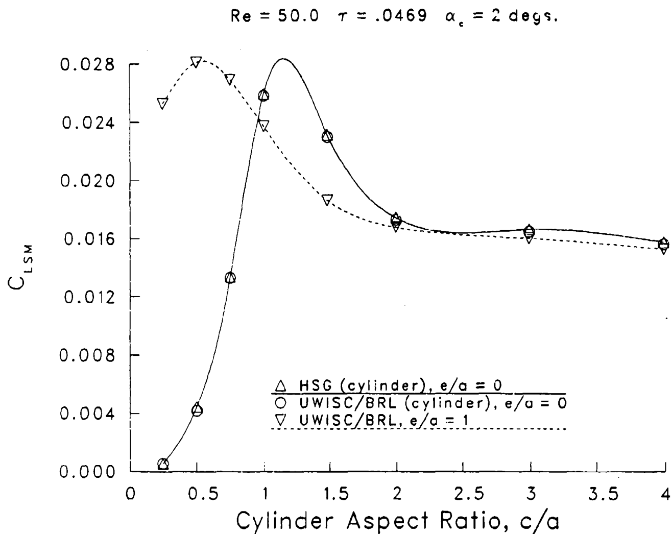
Figure 7. Variation of Liquid-Induced Side Moment Coefficient with Cylinder Aspect Ratio; e/a = 0 and 1 , Re = 50 , \tau = .0469 , \alpha_c = 2^\circ
