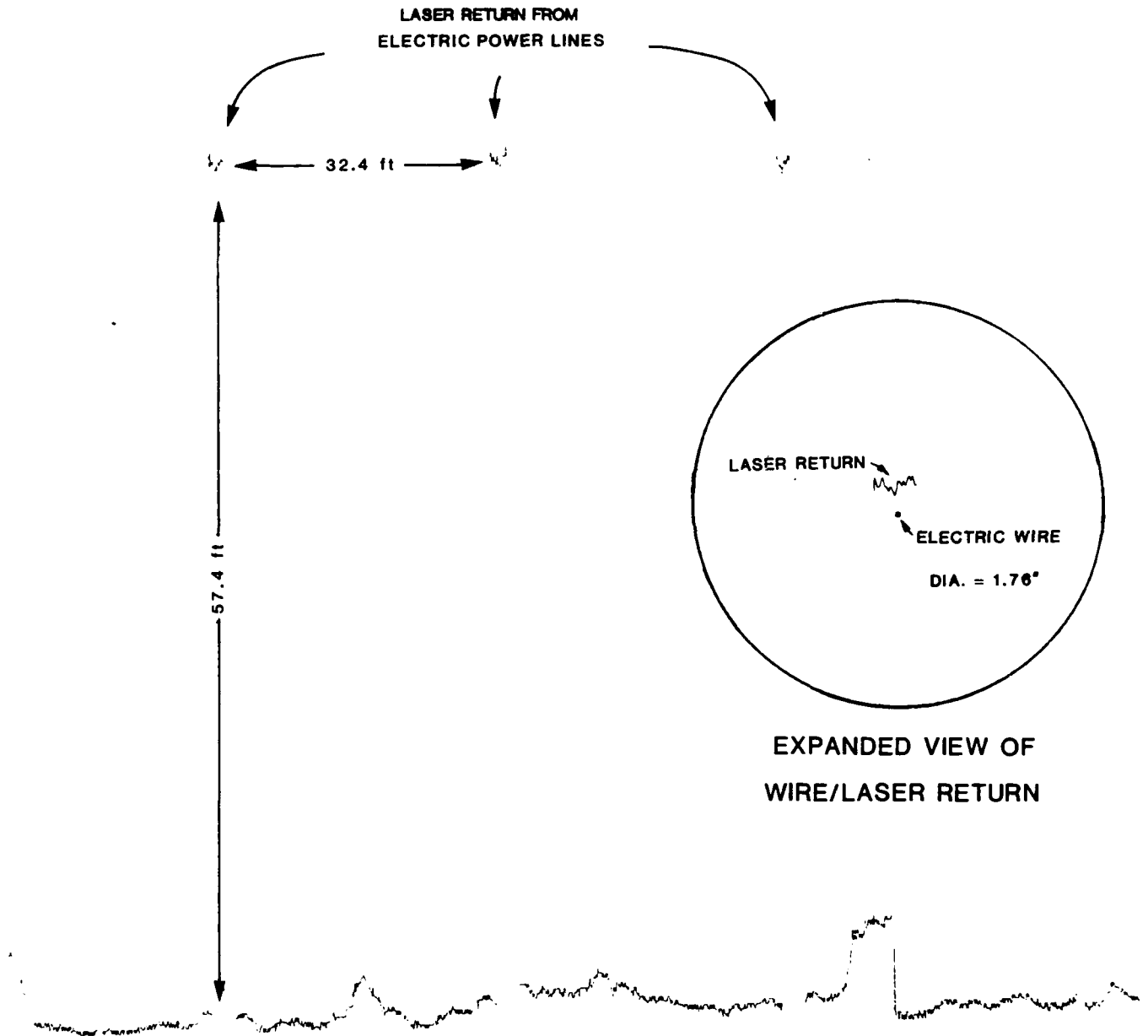
Figure 20. Laser profile of power lines.
