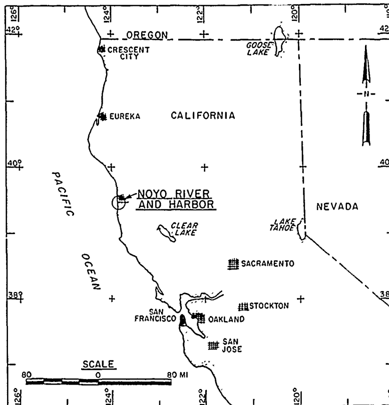
Figure 1. Project location
