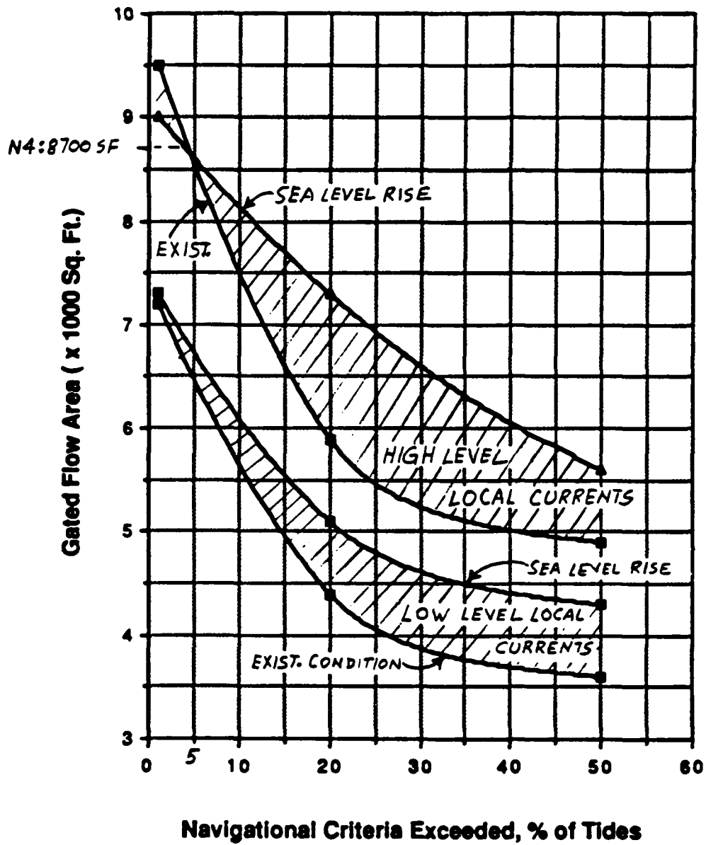
GRAPH F5 FLOW AREA VS. NAVIGATION CRITERIA
