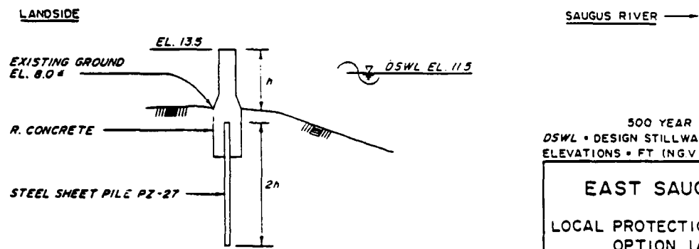
TYPICAL I-WALL - REACHES "C", "D", PART "B", "F"
