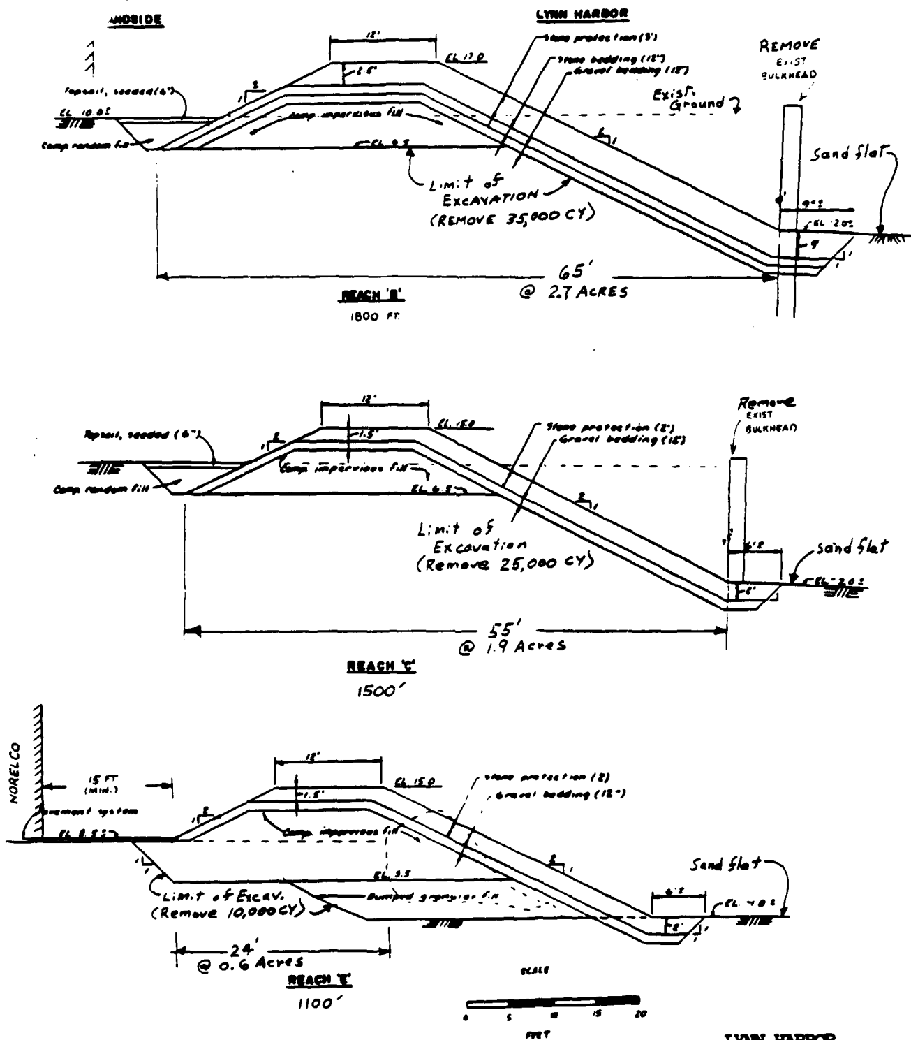
LYNN HARBOR Alternative #2 INLAND DIKES
